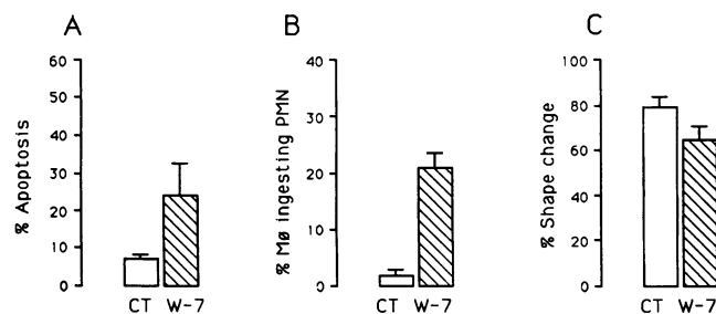
Figure 10. The effect of the calmodulin inhibitor, W-7 (60 \mu\text{M} ), upon neutrophil apoptosis, macrophage ingestion of neutrophils, and neutrophil function in vitro. In four experiments, neutrophils were incubated in the presence or absence of W-7 (60 \mu\text{M} ). Assessment of freshly-isolated (time 0) neutrophils in three of the four experiments showed 0.7 \pm 0.6\% apoptosis, 0.2 \pm 0.2\% macrophage ingestion, and 98.5 \pm 1.5\% stimulated change of shape. (A) After 8 h in culture, apoptosis was promoted in W-7-treated compared with untreated neutrophils ( P < 0.05 ). (B) At 8 h, W-7 had significantly increased macrophage ingestion of neutrophils ( P < 0.001 ). (C) Similar modulation of neutrophil ability to undergo change of shape upon stimulation ( P < 0.05 ).
