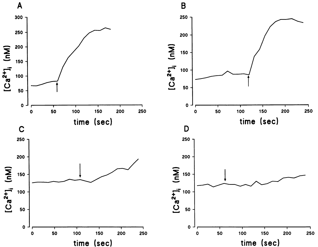
Figure 9. Measurements of resting cytosolic calcium levels and response to 1 \mu\text{M} 4-bromo A23187 in neutrophils preincubated for 8 h with various compounds. (A) Control, untreated cells ( 9.0 \pm 1.2\% apoptosis). (B) 1 \mu\text{M} 4-bromo-A23187 ( 1.2 \pm 0.6\% apoptosis). (C) 2.5 \mu\text{M} BAPTA/AM ( 27.0 \pm 3.3\% apoptosis). (D) 1 \mu\text{M} 4-bromo-A23187 and 2.5 \mu\text{M} BAPTA/AM ( 20.6 \pm 4.3\% apoptosis). 1 \mu\text{M} 4-bromo-A23187 was added to the cuvette as indicated by the arrows. These data, from a single experiment, are representative of three experiments.
