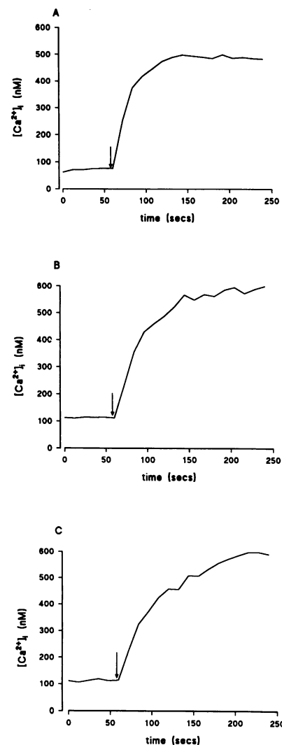
Figure 6. Cytosolic calcium levels in response to further addition of 1 \mu\text{M} 4-bromo-A23187. (A) Fresh neutrophils (0.8% apoptosis). (B) 20-h control (untreated) neutrophils (54.1% apoptosis). (C) 20-h 1 \mu\text{M} 4-bromo-A23187-treated neutrophils (19.2% apoptosis). Cytosolic calcium (nM) measured over 240 s, with 1 \mu\text{M} 4-bromo-A23187 added at 60 s, as indicated by the arrows. Cell populations obtained from a single donor. These data, from a single experiment, are representative of three experiments.
