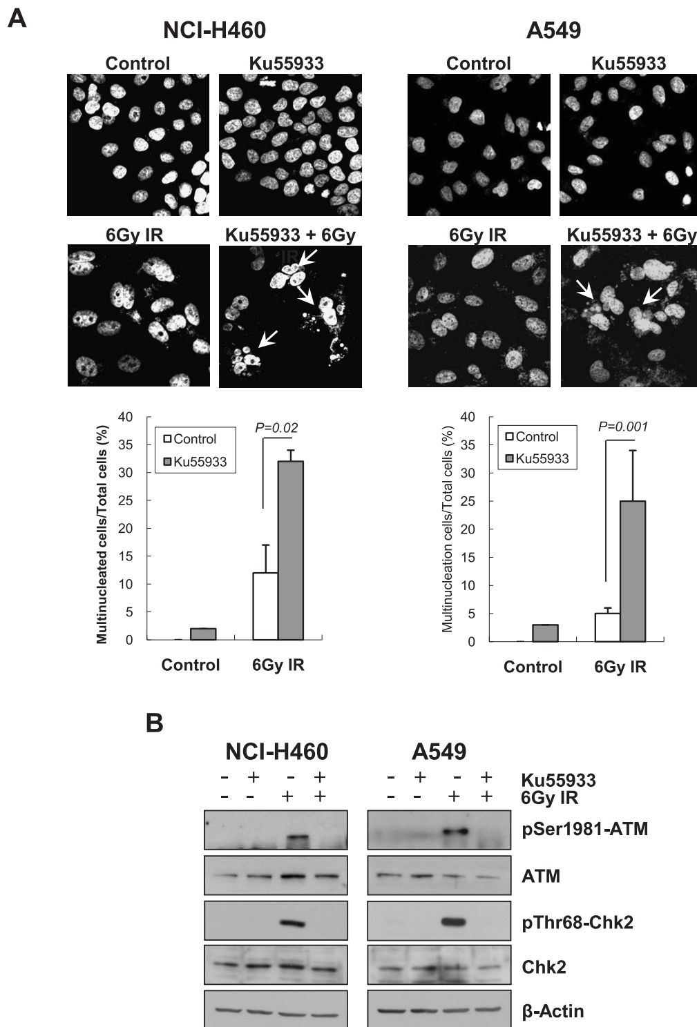
Figure 5 Induction of multinucleated cells after the treatment with Ku55933, a specific ATM inhibitor. A, NCI-H460 and A549 cells were grown on coverslips and treated with 10 \mu\text{mol/L} Ku55933 for 30 min and then exposed to 6 Gy ionizing radiation (IR). After 72 h, cells were fixed, stained with DAPI, and observed under confocal microscopy (X400). Cells with multinuclei were indicated with arrow. The number of multinucleated cells was counted and plotted. At least 100 cells were counted and each column represents the means of three independent experiments. Error bars , SE. B, Western blots after Ku55933 and IR treatment. Cells were pretreated with 10 \mu\text{mol/L} Ku55933 for 30 min, exposed to 6 Gy IR, and harvested after 30 min. Western blot analysis was done with anti-pATM, anti-ATM, anti-pChk2, anti-Chk2 antibodies. \beta -Actin was used as a loading control. Blots representative of three independent experiments.
