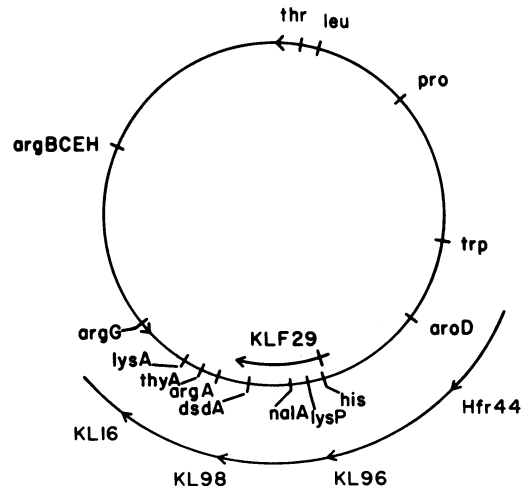
FIG. 4. Linkage map of E. coli with pertinent markers. For references to marker genes, see Bachman et al. (1); for origins of Hfr strains, see Low (20). nalA = gyrA .
