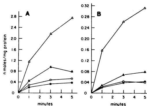
FIG. 2. Effect of pregrowth in the presence of 100 \mu\text{g} of L-lysine per ml on [ ^3\text{H} ]lysine uptake in JC182 and PSP01. Initial external lysine concentrations were 10^{-5} M (A) and 10^{-7} M (B). Symbols: \Delta , JC182 grown in minimal medium; \blacktriangle , JC182 grown in minimal medium plus 100 \mu\text{g} of L-lysine per ml; \circ , PSP01 grown in minimal medium; \bullet , PSP01 grown in minimal medium plus 100 \mu\text{g} of L-lysine per ml.
