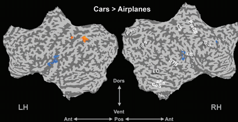
Figure 7. Experiment 2 intergroup comparisons. Experiment 2's group contrast (Experts vs. Novices) multisubject maps for the cars versus airplanes contrast in the high engagement condition (A) and the cars versus airplanes contrast in the low engagement condition (B), displayed on flattened cortical surfaces. These statistical maps show up the significant difference between the groups for the contrast specified ( P < 0.0001 , RE, corrected, minimum cluster size of 10 contiguous functional voxels). Experts: n = 13 , Novices: n = 14 ). Yellow to orange patches denote in (A) car-selective regions that were more activated in experts than in novices in the high engagement condition (i.e., defined by the contrast [\text{cars High Engagement} > \text{airplanes High Engagement}]_{\text{experts}} > [\text{cars High Engagement} > \text{airplanes High Engagement}]_{\text{novices}} ) and in (B) car-selective regions that were more activated in experts than in novices (i.e., defined by the contrast [\text{cars Low Engagement} > \text{airplanes Low Engagement}]_{\text{experts}} > [\text{cars Low Engagement} > \text{airplanes Low Engagement}]_{\text{novices}} ). The light blue patches denote regions exhibited negative results to these contrasts. Presentation format and anatomical landmarks as in Figure 2.
