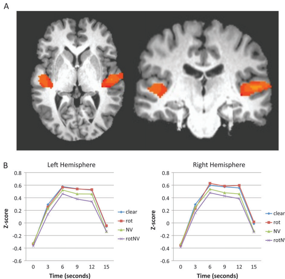
Figure 3. Activation of auditory core regions (HG) to 8-Hz amplitude-modulated wideband noise versus rest (scanner noise), P < 0.001 , uncorrected. (A) Axial and coronal slices showing activation in HG and immediately surrounding tissue. Images are in radiological convention (left = right). (B) Average signal time course for each speech condition for the HG ROI in each hemisphere. Note the virtually identical average response to clear and rot speech.
