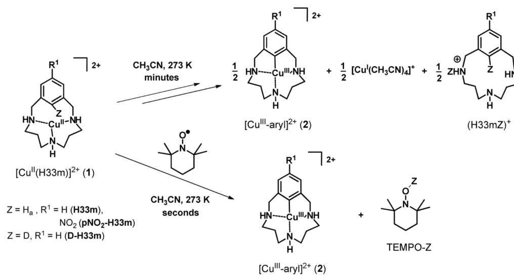
Figure 1. Facile C-H activation in the triazamacrocyclic ligands mediated by the reactivity of the C-H···Cu II species in the absence (upper reaction) or with the addition of TEMPO radical (lower reaction).
