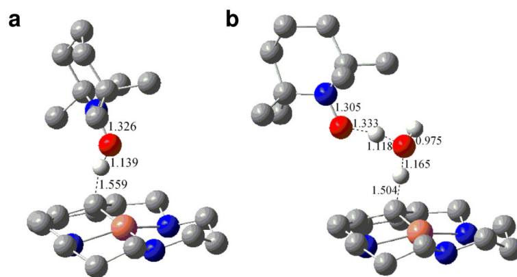
Figure 5. DFT optimization of transition states for (a) the bimolecular reaction between complex 1 and TEMPO with an energy barrier of 22.9 \text{ kcal mol}^{-1} , and (b) the same reaction assisted by an intervening water molecule with an energy barrier of 9.0 \text{ kcal mol}^{-1} .
