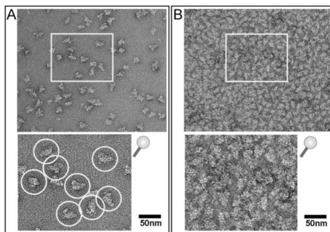
FIG. 4. Electron microscopic analysis of human U4/U6.U5 tri-snRNP complexes. A , negatively stained EM image of \sim 5 fmol of tri-snRNP per specimen. Individual particles showing the typical triangular shape of tri-snRNP can be distinguished ( upper panel , overview image; bottom panel , subwindow at a higher magnification as indicated in the upper panel ). Such a particle density is suitable for single particle image processing. Carbon films with adsorbed particles of this density were subjected to ECAD analysis. B , negatively stained EM image of tri-snRNP showing a particle density too high for image processing; exact counting of the particles is not possible at this high density ( upper panel , overview image; bottom panel , subwindow at a higher magnification as indicated in the upper panel ). Such a particle density is unsuitable for single particle image processing. These overloaded carbon films can in principle be analyzed by ECAD to increase the sample amount subjected to digestion; however, such overloading is not suitable for a correlation of the MS and EM analyses.
