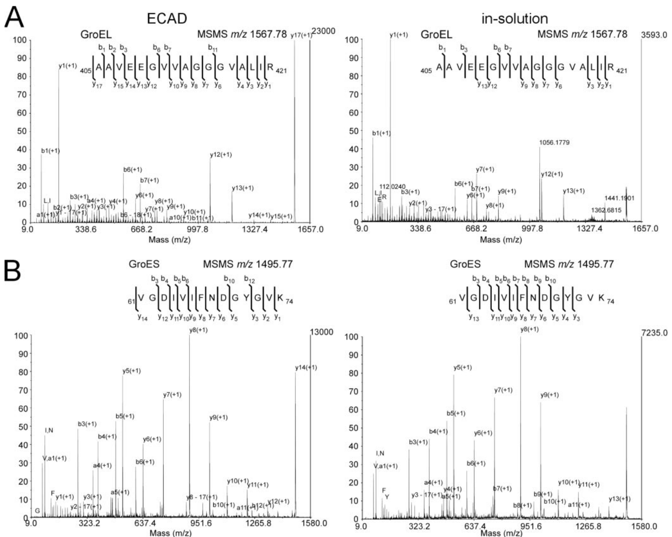
FIG. 5. MSMS spectra of GroEL-GroES using ECAD of fixed sample and in-solution digest of unfixed material. Shown is a collection of MSMS spectra that were derived from GroEL- (A) and GroES (B)-specific peptides upon fragmentation by CID. The spectra were selected from two comparable experiments using either 50 fmol of non-fixed material for in-solution digestion ( right ) or 50 fmol of glutaraldehyde-treated sample for ECAD ( left ). Both peptides displayed here were identified five times in five technical replicates. A, the MSMS-generated sequence information of the GroEL peptide AAVEEGVVAGGGVALIR (residues 405–421) is compared. The absolute intensity (and the signal-to-noise ratio) is higher by a factor of ~6.5. Sequencing of the ECAD-generated peptide derives an almost complete coverage of the y-type ion series. B, similar results were observed for the GroES-specific peptide VGDIVFNDGYGVK (residues 61–74); the absolute ion intensity was higher by a factor of 1.8.
