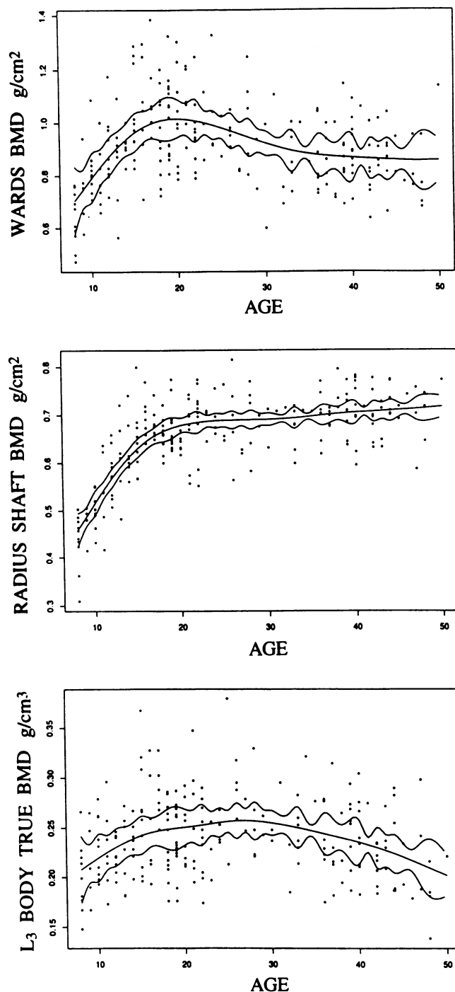
Figure 1. Cubic splines with 95% pointwise confidence interval for various BM-age profiles. From top to bottom: Ward's BMD profile over time representative of quadratic-quadratic model; BMD of the radius representing quadratic-linear model; and true density of the vertebral body representing single quadratic model.
