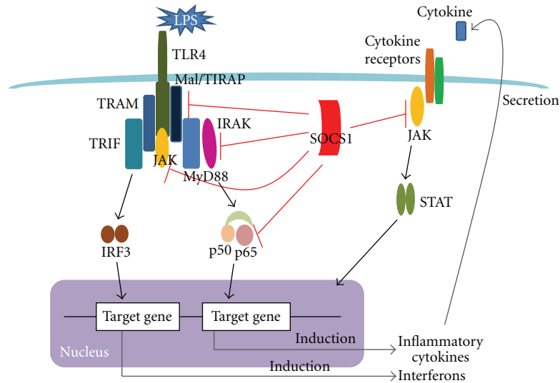
FIGURE 2: Proposed inhibitory mechanisms of SOCS1 on TLR signaling. The absence of SOCS1 results in heightened response to TLR ligands. Possible mechanisms of action of SOCS1 proposed so far are outlined here. Upon induction, SOCS1 binds to Mal/TIRAP and mediates its degradation via proteasomal pathway (1). SOCS1 binds to IRAK and may modulate its activity (2). SOCS1 binds to p65 subunit of NF \kappa B and targets it for proteasomal degradation (3). SOCS1 inhibits JAK2 activated directly after TLR stimulation (4). SOCS1 regulates TLR-mediated response indirectly by inhibition of TLR-induced cytokines such as IFN- \beta (5).
