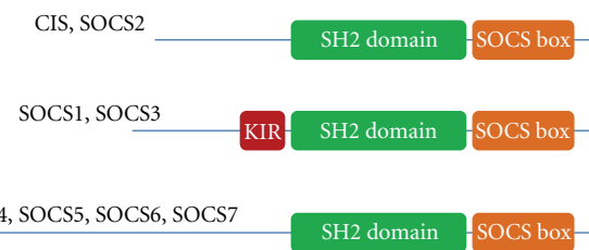
FIGURE 1: Schematic structure of SOCS proteins. SOCS proteins are structurally characterized by a central SH2 domain, a docking motif to tyrosine-phosphorylated proteins, and a c-terminal SOCS box that recruits Elongin B/C complex. SOCS1 and SOCS3 also possess a KIR domain, which plays an important role in inhibition of JAK kinase activity. The length of N-terminal domain varies between SOCS proteins and SOCS4-7 possesses relatively long N-terminal domain.
