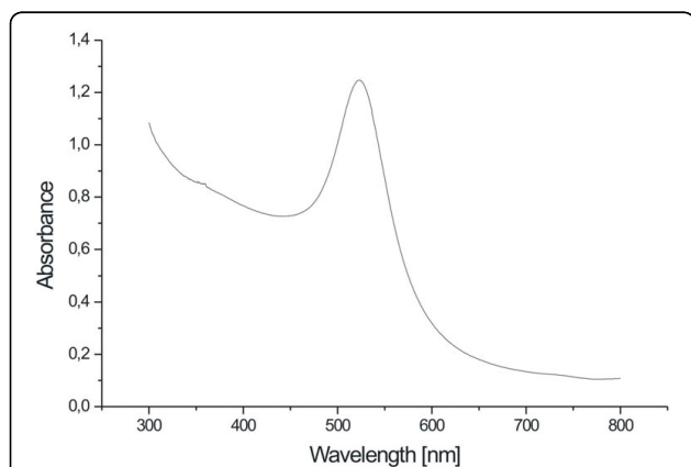
Figure 2 UV/VIS spectrum of aptamer-conjugated AuNPs. The spectrum was obtained with an as prepared AuNP solution after in situ conjugation with 5 μM anti-streptavidin aptamer.
