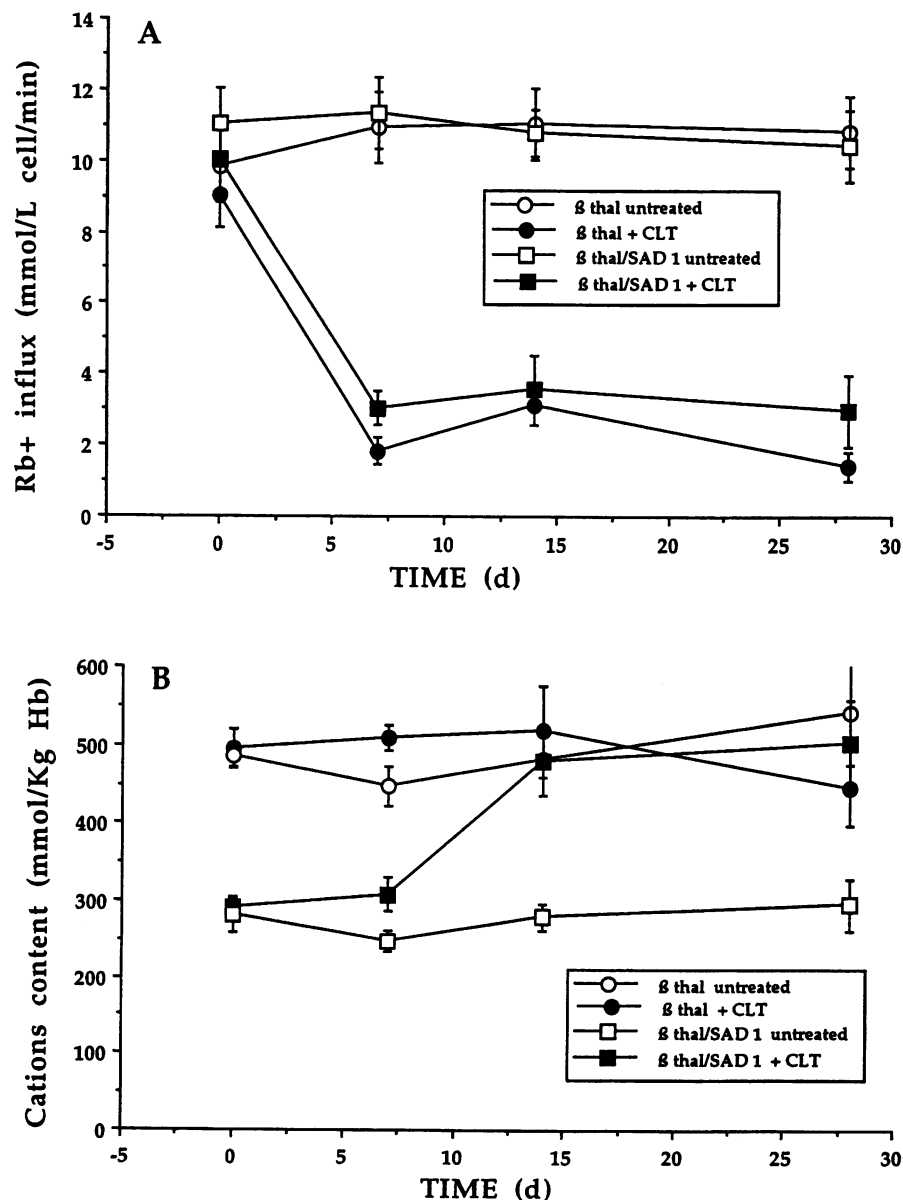
Figure 4. In vivo effect of long-term treatment (28 d) with oral CLT (80 mg/kg per d) and with the suspension medium without CLT in transgenic ( Hbb^{\beta}/Hbb^{thal} SAD 1) and control ( Hbb^{\beta}/Hbb^{thal} ) mouse red cells. (A) Effect on Ca^{2+} -activated Rb^+ influx. (B) Effect on intracellular K^+ content. The data are expressed as means±SD ( n = 6 ).
