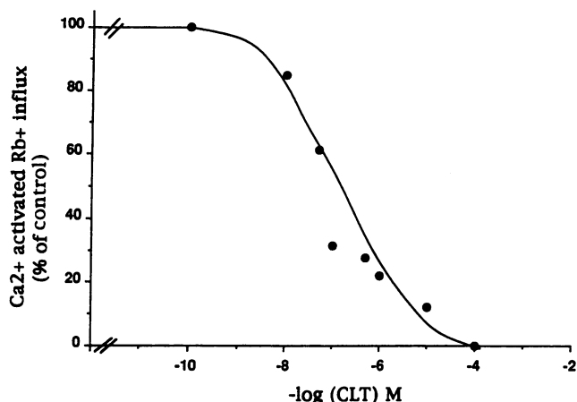
Figure 1. Inhibition of \text{Ca}^{2+} -activated \text{Rb}^{+} influx in transgenic ( \text{Hbb}^{\text{S}}/\text{Hbb}^{\text{thai}} SAD 1) mouse red cells by increasing concentrations of CLT. Data points represent mean values of three separate experiments. Curves were computer-fit using a logistic dose-response model. SD for all the data points was between 5 and 15% of the mean values.
