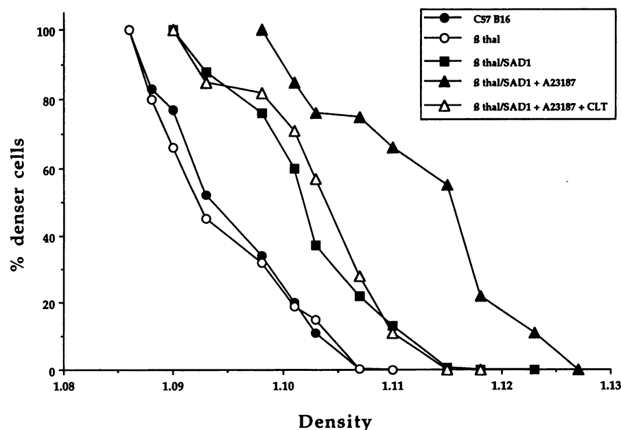
Figure 2. Phthalate density profiles portraying the effect of 10 mM CLT on the dehydration of transgenic ( \text{Hbb}^{\text{S}}/\text{Hbb}^{\text{thai}} SAD 1) mouse red cells via A23187-induced activation of the \text{Ca}^{2+} -dependent \text{K}^{+} channel. Data are from one experiment, representative of three separate experiments.
