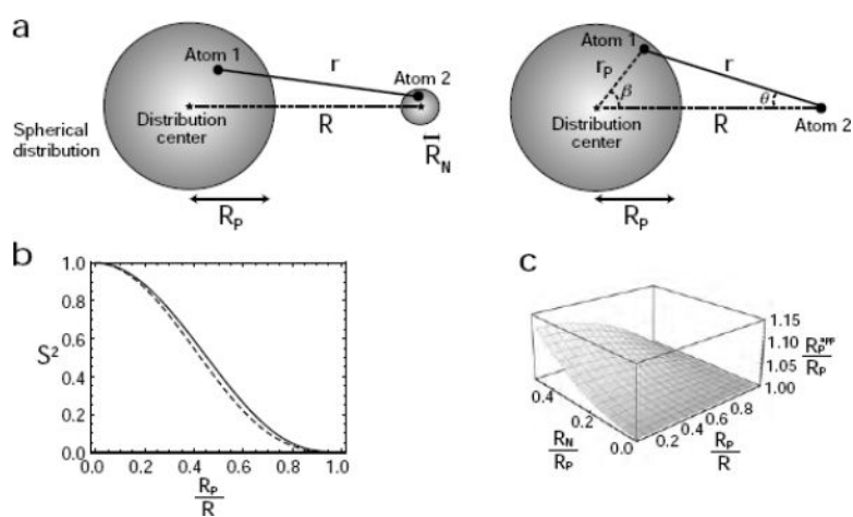
Figure 2. 'Sphere' model for the internal motion of a variable-length vector in a macromolecular system. (a) Diagram depicting the DIS model in which atoms 1 and 2 are uniformly distributed in two separate spheres. On the left, atom 2 is distributed in a sphere of radius R_N ; on the right, the case with R_N = 0 is shown. (b) Relationship between the order parameter S^2 for the variable-length vector and the ratio R_p/R for the 'Sphere' model (solid line, R_N = 0 ; dotted line, R_N/R_p = 0.4 ). (c) Impact of neglecting R_N in the determination of R_p . The ratio of the apparent R_p (obtained from Eqs. [4], [7] and [8]) to the true value of R_p as a function of R_p/R and R_N/R_p is plotted.
