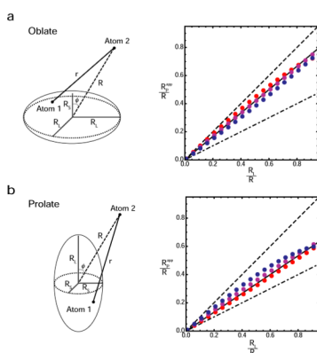
Figure 3. Calculated value of the apparent distribution radius R_P^{app} for oblate (a) and prolate (b) axially symmetric ellipsoids. Five parameters are involved: the lengths of the axes R_L and R_S ( R_L > R_S ), the angle \phi between the symmetry axis and the center – Atom 2 vector, the distance R between the center of an ellipsoid and Atom 2, and the distance r between Atom 2 and an arbitrary position in the ellipsoid. The order parameters S^2 and effective distances \langle r^{-6} \rangle^{-1/6} were calculated using 3581 uniformly distributed grid points for an oblate ellipsoid and 3591 grid points for a prolate ellipsoid. Graphs display apparent R_P/R values (red points, \phi = 90^\circ ; magenta, \phi = 45^\circ ; and blue, \phi = 0^\circ ) as a function of the R_L/R ratio for oblate and prolate ellipsoids with an anisotropy of R_L/R_S = 2.0 . Dotted and dashed lines correspond to R_L/R and R_S/R , respectively. Solid lines represent (2R_L/3 + R_S/3)/R for an oblate ellipsoid, and (R_L/3 + 2R_S/3)/R for a prolate ellipsoid.
