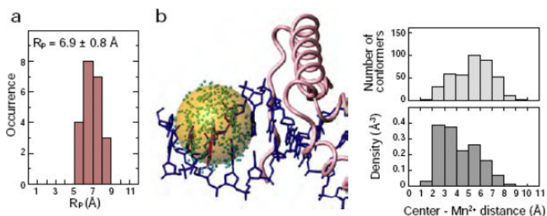
Figure 8. The distribution radius R_p of the EDTA-Mn 2+ group in the SRY/DNA complex. (a) Histogram of R_p calculated from S^2 and \langle r^{-6} \rangle^{-1/6} for 22 Mn 2+ - 1 H vectors in the SRY/DNA-EDTAMn 2+ complex. (b) Mn 2+ distribution obtained by structure-based simulated annealing calculations. In the left panel of (b), the positions of Mn 2+ for 400 different conformers are shown in green. The transparent orange sphere, with its origin placed at the center of the distribution, is drawn with a radius of 6.9 Å, corresponding to the average value of R_p determined by the structure-independent method. In the right-hand panel of (b), a histogram of the distance from the center of the distribution to individual Mn 2+ positions (top) and the density (bottom) of the Mn 2+ for the 400 conformers (obtained by dividing the number of conformers by the volume of a shell with 1 Å thickness) are shown.
