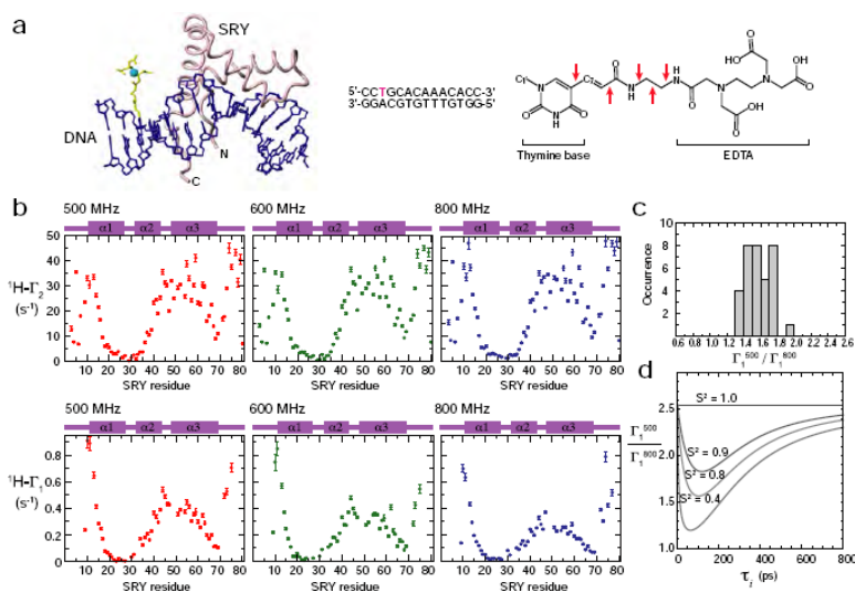
Figure 6. PRE measurements for the SRY/DNA complex at multiple fields. (a) Structure of the SRY/DNA-EDTA-Mn 2+ complex. 17 The EDTA-Mn 2+ group (yellow/cyan) is tethered to a thymine base (red in the sequence) in the 14-bp DNA duplex. The chemical structure of T-EDTA is also shown (asterisks, coordination sites; arrows, rotatable bonds in the linker). (b) PRE 1 H-N-Γ 1 and Γ 2 rates measured at three magnetic fields. (c) Histogram of the ratio of PRE 1 H-N-Γ 1 rates measured at 500 and 800 MHz. (d) Theoretical dependence of Γ 1 500 /Γ 1 800 ratio on the order parameter S 2 and the internal motion correlation time τ i for a Mn 2+ - 1 H vector.
