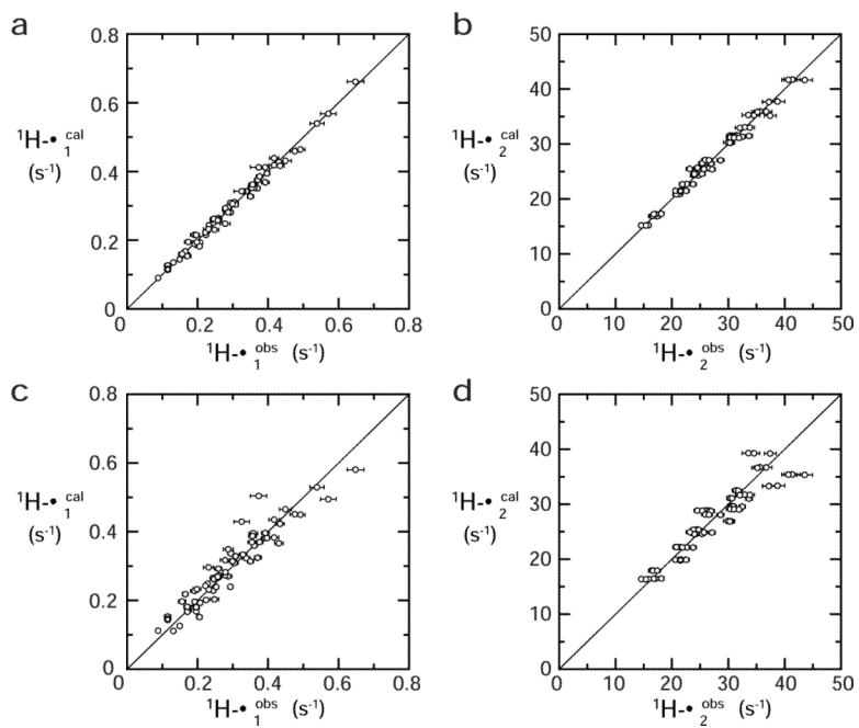
Figure 7. Correlation between calculated and observed PRE rates. (a, b) Fitting Procedure 1. (c, d) Fitting Procedure 2. Statistics are given in Table 1.
