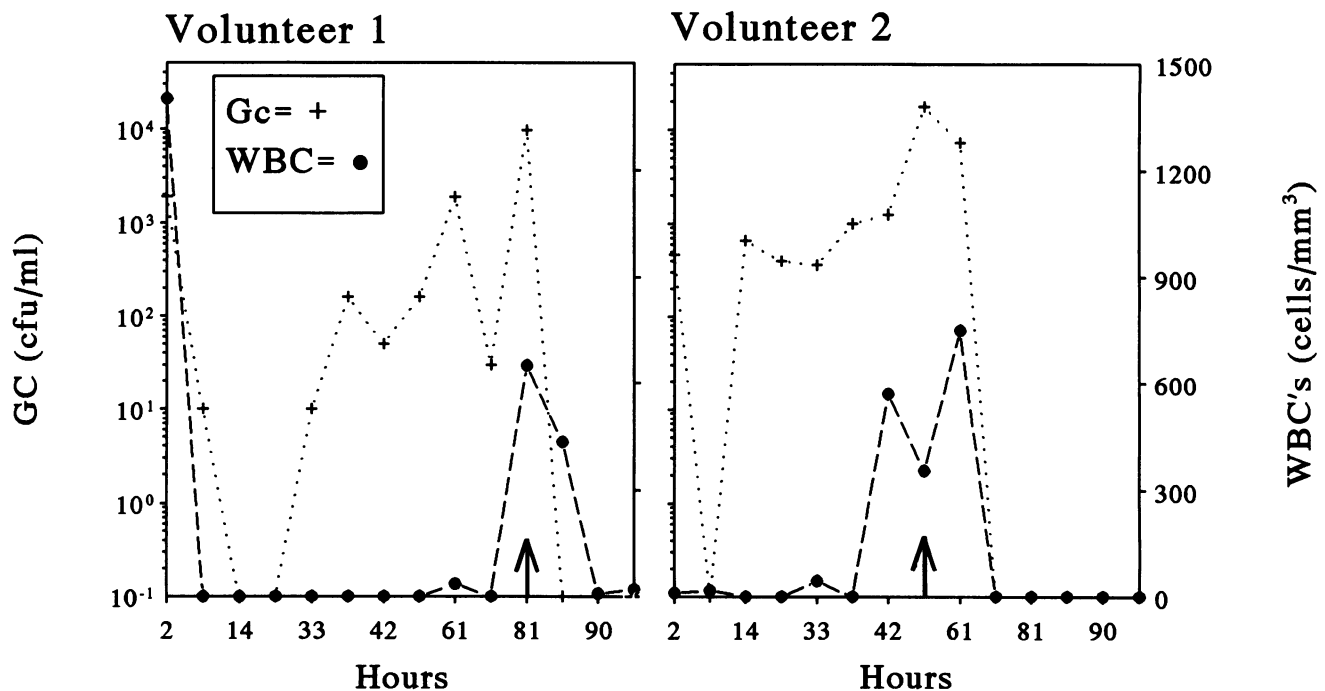
Figure 1. Time course of human volunteer infection. \sim 1.2 \times 10^6 colony forming units (cfus) of the same culture were inoculated intraurethrally in each volunteer at time zero as described (25). At the times after inoculation, Gc cfu's or WBCs in resuspended urine sediments were quantified. Data for Gc are expressed as cfu/ml of resuspended urine sediment and WBCs as cells/mm 3 of resuspended urine sediment (note: samples with zero cfu are represented as 10 -1 on the log scale). The arrow shows when clinical signs of disease were recorded and antibiotic treatment was administered.
