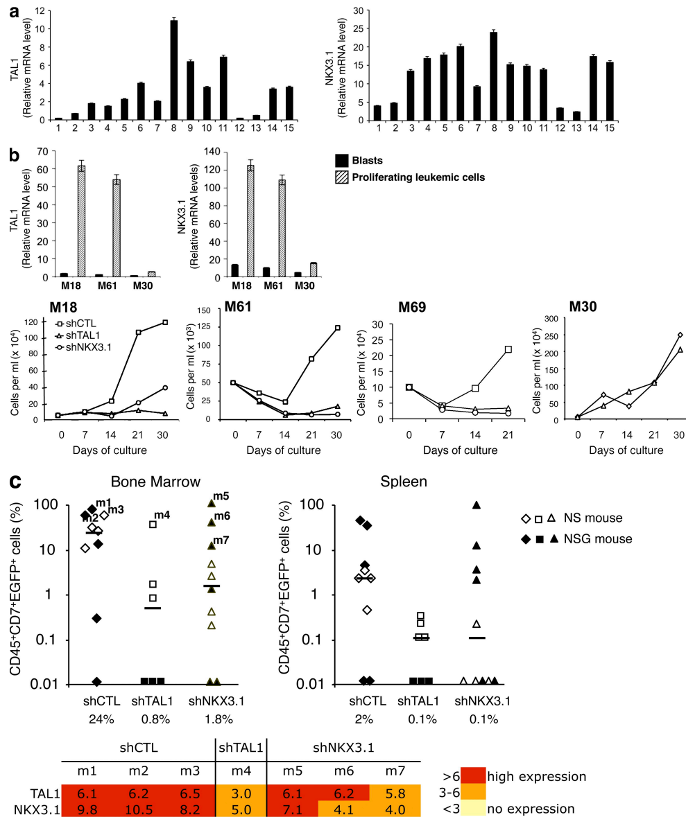
Figure 8. NKX3.1 is expressed in human TAL1-expressing T-ALL cells and is necessary for in vitro proliferation and in vivo development of human T-ALL. (a) TAL1 and NKX3.1 mRNA levels in human T-ALL blasts at diagnosis. Quantitative RT-PCR analysis of TAL1 and NKX3.1 mRNA was performed using RNA prepared from blasts obtained from 15 human T-ALL. Relative expressions were normalized to \beta 2m mRNA. Error bars represent means \pm SEM ( n = 4 experiments). (b, top) TAL1 and NKX3.1 mRNA levels were analyzed by quantitative RT-PCR using RNA extracted from TAL1-expressing (M18 and M61) or non-TAL1-expressing (M30) T-ALL leukemic cells at diagnosis (black bars) or after 3 d of culture on the MS-5 cell line expressing the DL1 Notch ligand (MS5-DL1; hatched bars). Relative expressions were normalized to \beta 2m mRNA level. Error bars indicate SEM ( n = 4 experiments). (bottom) Growth curves of M18, M61, M69, and M30 primary T-ALL expressing shCTL, shTAL1, or shNKX3.1 co-cultured with MS5-DL1 for 21 d (M69) or 1 mo. (c) M18 leukemic cells expressing shCTL, shTAL1, or shNKX3.1 were injected into NS and NSG mice. (top) Percentages of human leukemic transduced (CD45 + CD7 + EGFP + ) cells detected in bone marrow and spleen of mice at 6 (NSG) and 12 (NS) wk after transplantation. Median engraftment levels (horizontal bars) are indicated under the diagram. (bottom) Quantitative RT-PCR analyses of TAL1 and NKX3.1 mRNA were performed using RNA from CD45 + CD7 + EGFP + cells isolated from mice that developed leukemia (m1–m7). Relative expression levels were normalized to \beta 2m mRNA level and represented by a color scale ( n = 3 experiments).
