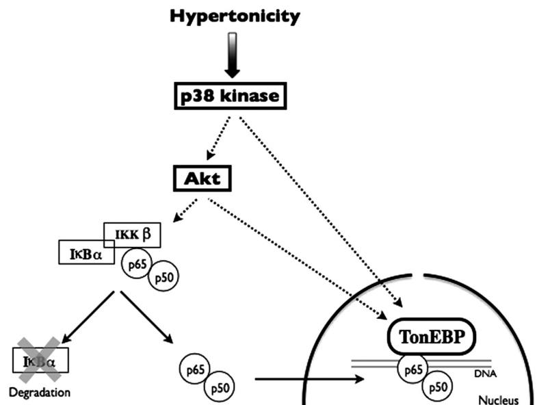
Figure 10. Proposed mechanism for NF- \kappa B activation by hypertonicity. Hypertonicity activates NF- \kappa B in a two-step process. In a first step, hypertonicity stimulates p38 kinase, which enhances the activities of both Akt and TonEBP. Increased Akt activity in turn not only contributes to enhancing TonEBP activity but also induces I \kappa B \alpha to dissociate from cytosolic p65. This process depends on IKK \beta activity. Unconjugated I \kappa B \alpha is degraded allowing free p65, associated with other NF- \kappa B binding partners such as p50, to translocate across the nuclear membrane. In a second step, TonEBP associates with p65-containing complexes bound to DNA, enhancing NF- \kappa B transcriptional activity. NF- \kappa B activation by hypertonicity is transient and decreases as I \kappa B \alpha protein expression increases in response to increased I \kappa B \alpha transcriptional activity.
