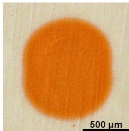
Fig. 4. Optical images of the colorimetric sensor array of porous pigments. Left, scanned image from a flat bed scanner; right, microscopic image of a single pigment spot.
