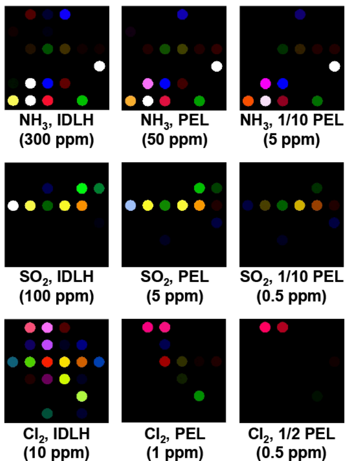
Fig. 5. Color difference maps (averages of five trials each) of three toxic gases at different concentrations after 2 min of exposure. For purposes of visualization, the color range of these difference maps are expanded from 4 to 8 bits per color (RGB range of 4-19 expanded to 0-255). From the S/N ratio of the total Euclidean distances of these difference maps at the lowest concentrations tested, the estimated limits of detection are well below 100 ppb for each of these analytes.
