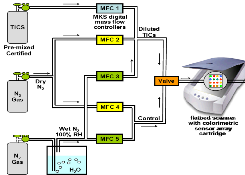
Fig. 1. Experimental setup for the gas mixing of TICs and digital imaging of arrays
