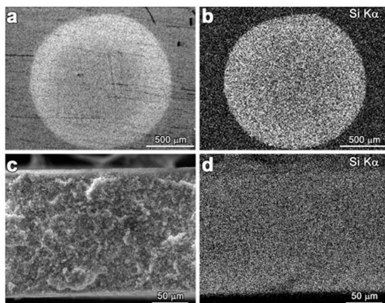
Fig. 3. SEM micrographs PVDF printed with a 1.5 mm spot of sol-gel porous pigment: (a) top surface and (b) EDS elemental mapping (Si K \alpha ) of top surface; (c) cross-section and (d) EDS elemental mapping (Si K \alpha ) of cross-section.
