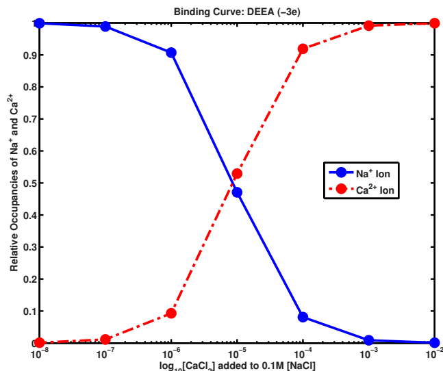
FIG. 2. Binding of calcium to a DEEA channel. This figure shows the relative occupancy of the cylindrical space, that is to say, it shows the ratio of the spatial integral of the density of calcium (diameter of 1.98 Å) to the spatial integral of the density of sodium (diameter of 2.04 Å)—both within a cylindrical space of 3.5 Å radius and 3 Å length—of the stationary solution of the time dependent Euler–Lagrange equations. The concentration of sodium is maintained at 0.1 M on both sides of the channel. The concentration of calcium is varied and is shown on the horizontal axis. The dielectric constant was 80 and the temperature was 298 K. Geometrical setup is nearly the same as Figs. 1 and 2 of Ref. 15.
