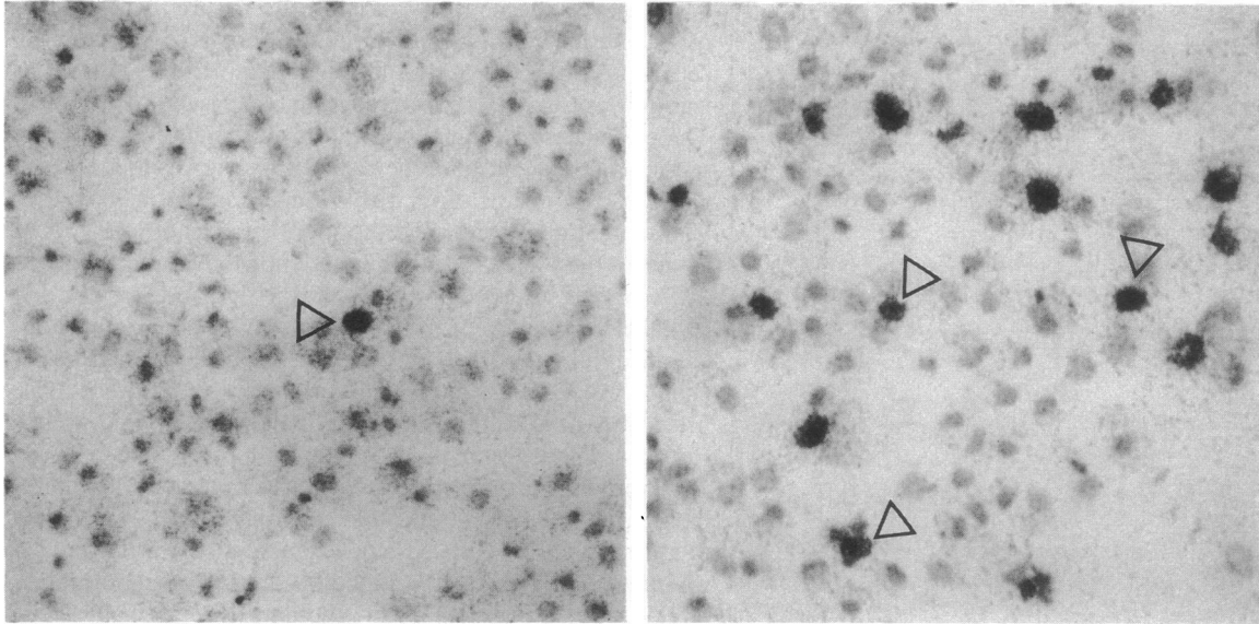
Figures 1 and 2. Autoradiographs of a cytospin preparations prepared from human T cell clone before (left) and after (right) stimulation with con A. In situ hybridization was performed with ^{32}\text{P} -labeled IL-5 cRNA probe. Arrows indicate the positive IL-5 mRNA signals. Note the difference in the number of IL-5-positive cells. Magnification for Fig. 1 and 2, 400.
