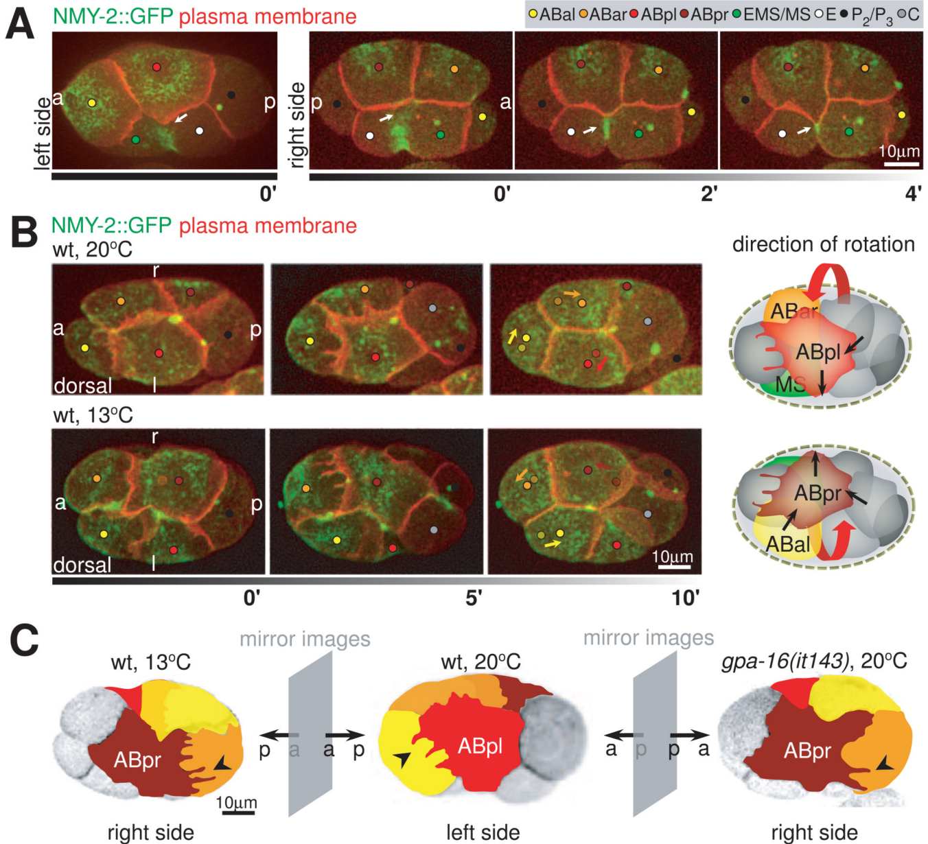
Figure 5. Handedness of Chiral Morphogenesis
