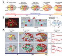
Figure 1. Formation of a Midline through Blastomere Rearrangements
