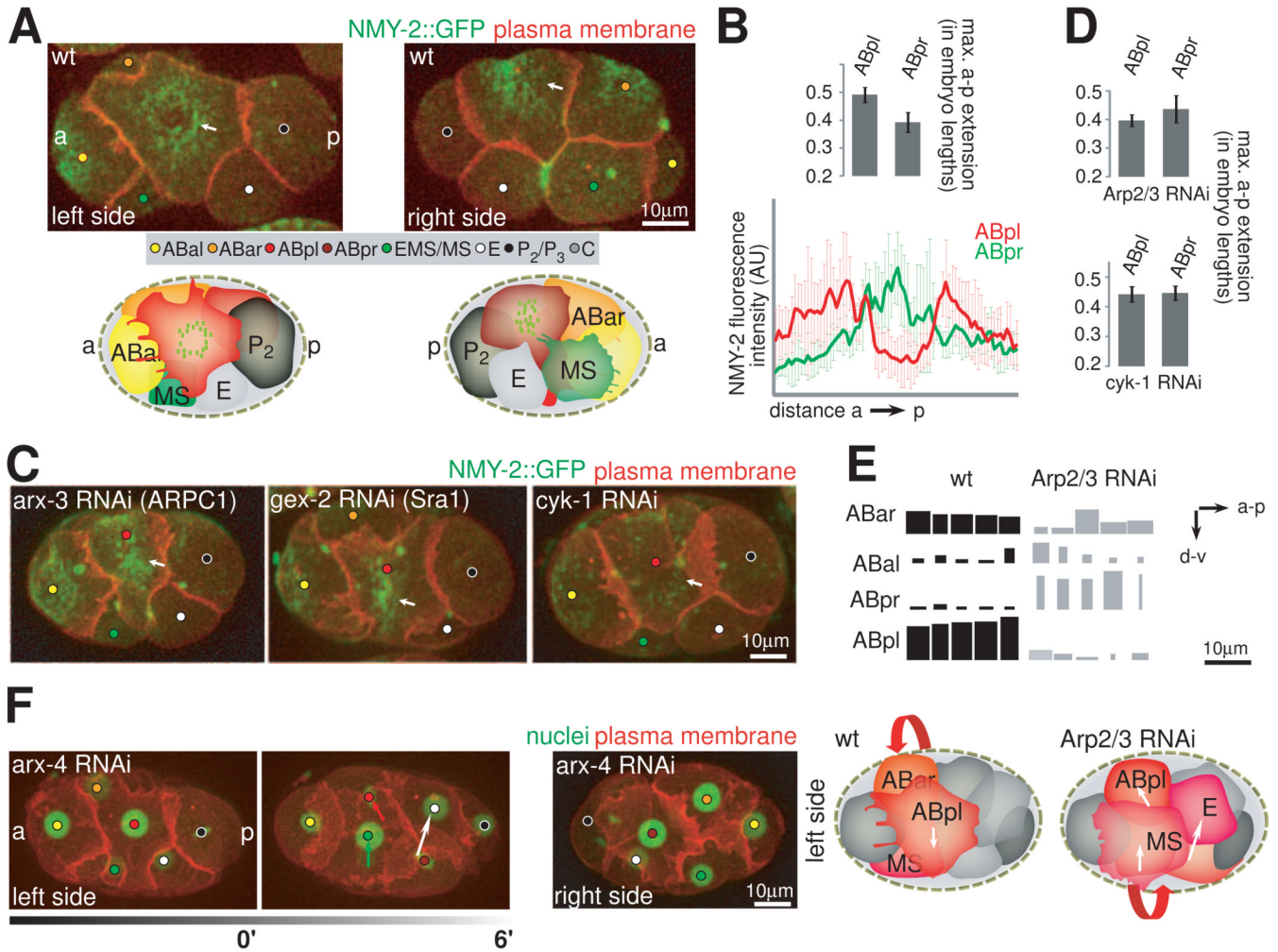
Figure 6. LR Asymmetries in ABpl/pr Cortical Contractility A. Asymmetry of the apical NMY-2 cap structure. 3D-projection stills, left side and right side views with matched schematics. Plasma membrane is shown in red and the actomyosin cortex (NMY-2::GFP) in green. Arrows point to the center of the cap structure on the respective sides. Green speckles in the cartoons indicate the distribution of cortical contractile elements on either side of the embryo. See also Movie S9. B. Quantification of the AP extension of ABpl and ABpr and of the cortical NMY-2 signature. Upper panel: AP extensions of the respective cells were measured from time-lapse microscopy data and normalized to the length of the respective embryo (n=10, mean +/- SD). Lower panel: Graphs displaying cortical NMY-2::GFP fluorescence intensity as measured on a line parallel to the AP axis that transects the center of ABpl (red) and ABpr (green), respectively (n=3, mean +/- SD). C. Perturbations of actomyosin and its consequences for asymmetric cortical dynamics. Representations as in A. Wt and embryos treated with RNAi targeting the indicated genes are shown. Arrows point to the center of the apical surface of ABpl. D. Loss of differential LR surface occupancy in Arp2/3 and cyk-1 RNAi embryos. Graph showing AP extensions as in B for the respective RNAi-treated embryos (n= 5, mean +/- SD). For details on protrusion formation see Figure S3C. E. Nuclear migration paths in wild-type and Arp2/3 RNAi embryos. Displacement of AB nuclei in AP and DV direction during chiral morphogenesis are shown as boxes for 5 wild-type and 5 Arp2/3 RNAi embryos with inverted handedness of collective rotation. Boxes are
