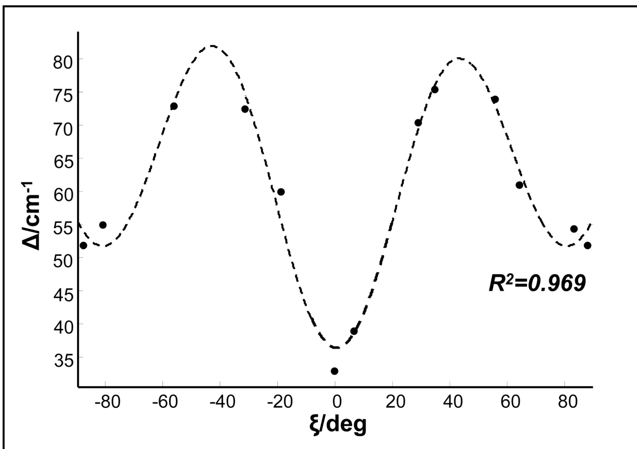
Figure 8. Calculated \xi angular dependence of frequency splitting of the gly \text{CH}_2 stretching. The dots represent calculated data points, the dashed line is the Fourier fit to the calculated results. \Delta(\xi) = 60 - 10.6\cos(0.04\xi) - 4.3\sin(0.04\xi) - 21.3\cos(0.08\xi) - 3.6\sin(0.08\xi)
