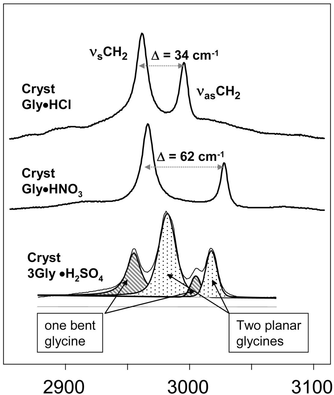
Figure 2. Raman spectra of the CH stretching region of the crystalline gly hydrochloride (Gly•HCl), crystalline gly nitrate (Gly•HNO 3 ), crystalline trigly sulphate or TGS (3Gly•H 2 SO 4 ).
