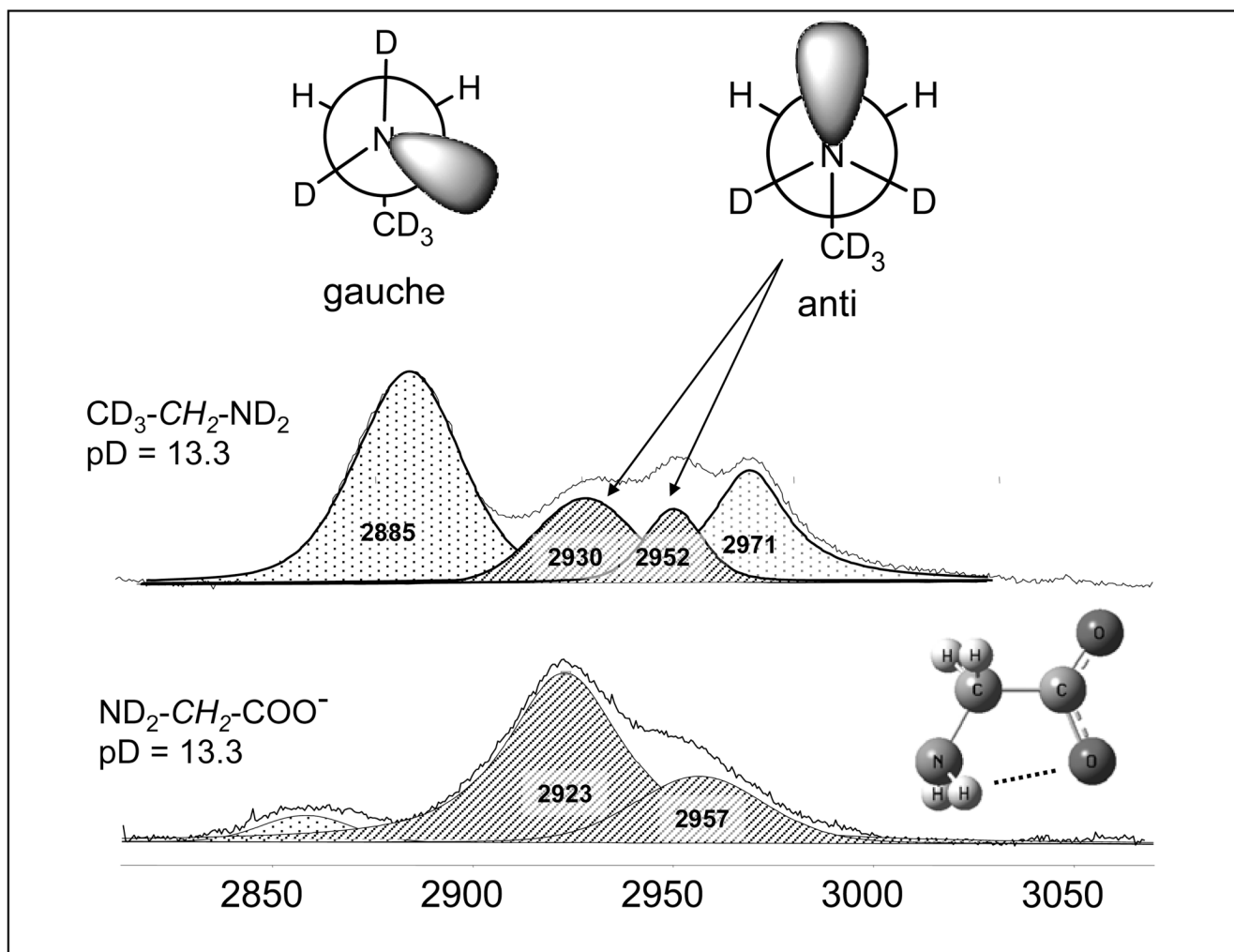
Figure 9. Fitted Raman spectrum (CH 2 stretching region) of the CD 3 -CH 2 -ND 2 and ND 2 -CH 2 -COO - solutions in D 2 O at pD = 13.3. Also shown are the two conformations of the ethylamine and for gly - in solution.
