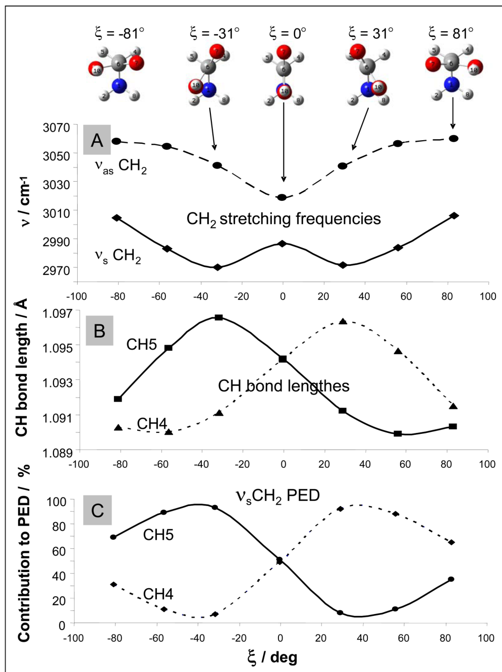
Figure 7. Calculated \xi angular dependence of (A) gly CH 2 stretching frequencies, (B) C-H bond lengths, and (C) normal mode composition (%) of CH 2 symmetric stretch. Frequencies are scaled to 0.98.
