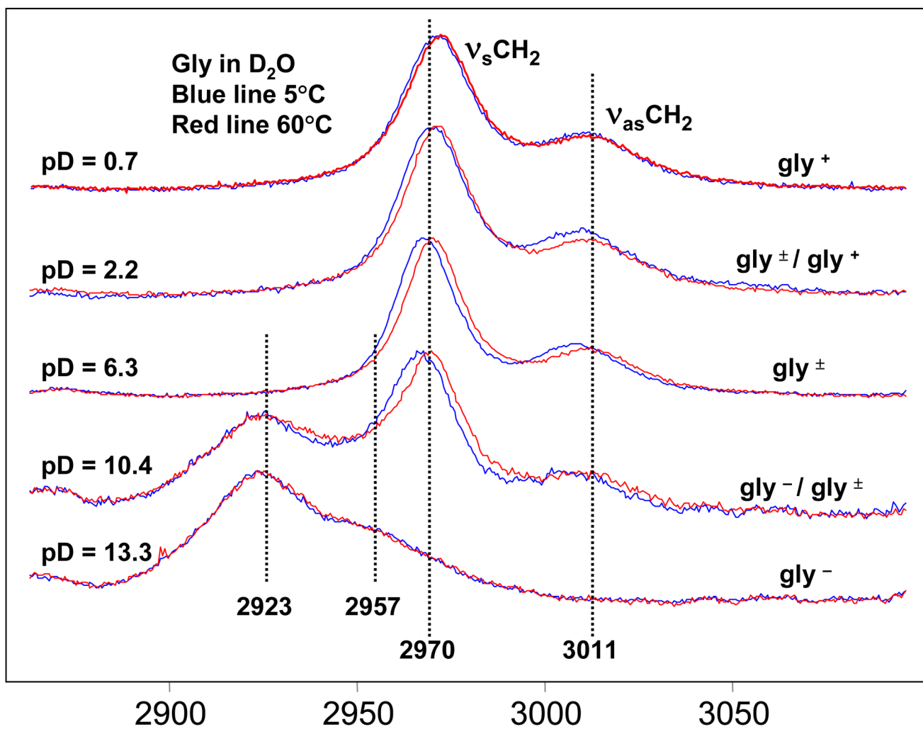
Figure 4. 488 nm excitation Raman spectra of gly solution in D 2 O at pD= 0.7, 2.2, 6.3, 10.4, 13.3. For each solution spectra were accumulated at two temperatures 5°C and 60°C.
