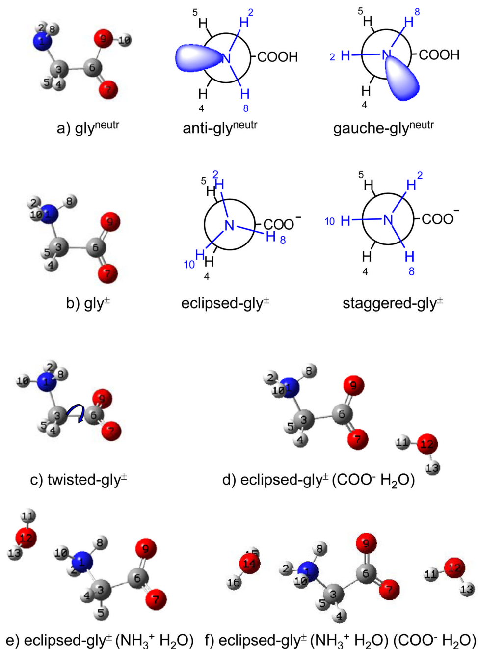
Figure 1. Calculated conformers of gly: a) anti and gauche rotamers of neutral gly; b) eclipsed and staggered rotamers of zwitterionic gly; c) non-planar conformer ( \xi = 60^\circ ) of zwitterionic gly; d) eclipsed zwitterionic gly hydrogen bonded to the acceptor water molecule, e) eclipsed zwitterionic gly hydrogen bonded to the donor water molecule, f) eclipsed zwitterionic gly hydrogen bonded simultaneously to the acceptor and donor water molecules. All conformers except c) are planar \xi = 0^\circ .
