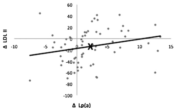
Fig. 2. Spearman's correlation between diet-induced changes in lipoprotein(a) [Lp(a)] (mg/dl) and medium-size LDL II particles (mg/dl). n = 62 , r = 0.34 , P < 0.01 . The value corresponding to mean changes in Lp(a) and LDL II is shown by \times .
