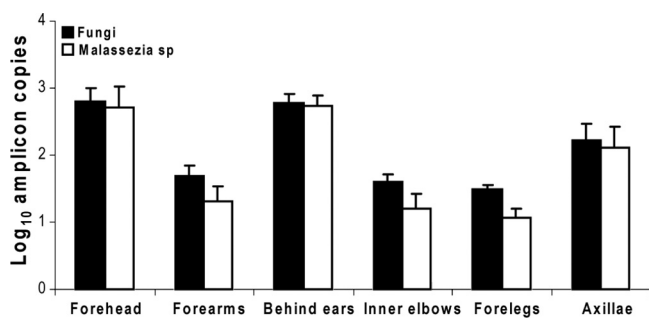
FIG. 3. Enumeration of fungal species in six cutaneous locales. From the eight tested subjects, a single specimen was obtained from the forehead and bilateral specimens were obtained from forearm, behind ear, inner elbow, and foreleg; samples from axillae were obtained for five subjects only. qPCR was performed using primers for universal fungal or Malassezia species. Bars indicate mean \pm SD of the values across the subjects. The data were not normalized with respect to the human GAPDH gene.
