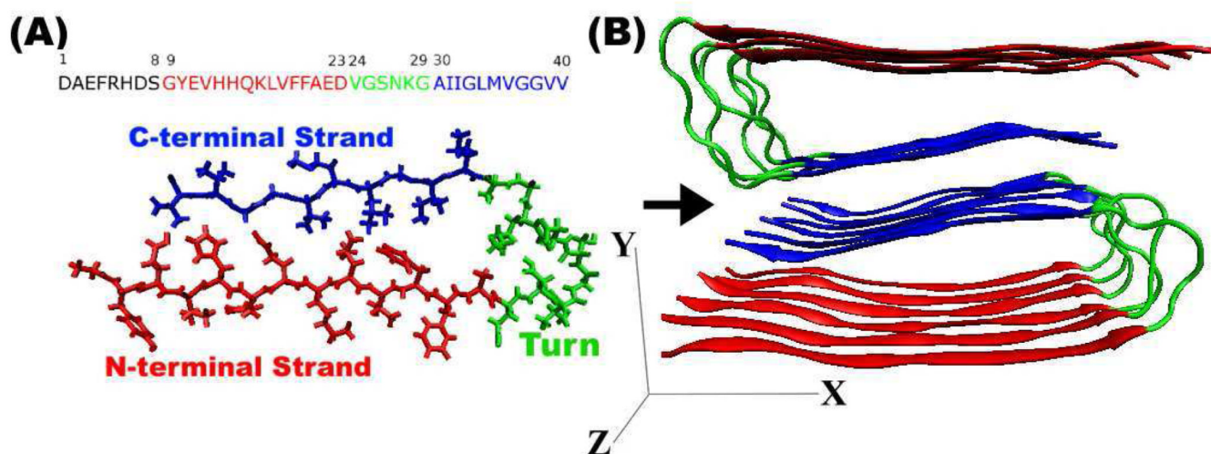
Figure 1. (A) Aβ 1-40 sequence and the structure of a single Aβ 9-40 peptide, with asymmetric “U” structure. N-terminal strand (red), C-terminal strand (blue), and turn region (green), respectively. (B) Model structure of amyloid fibril made of 12 Aβ 9-40 molecules. Red and blue indicate two parallel β-sheets.
