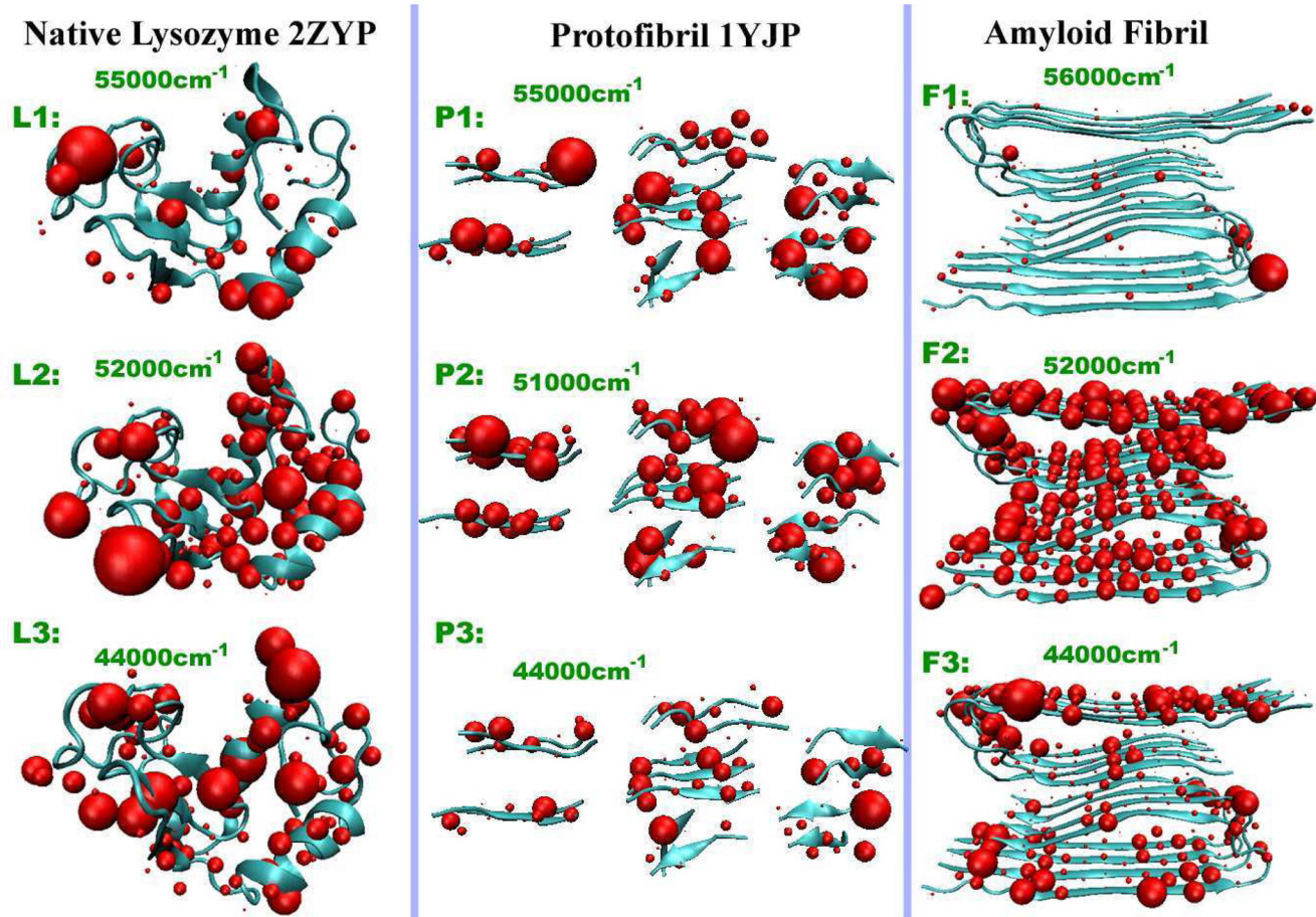
Figure 3. Transition populations of native lysozyme 2ZYP, protofibril 1YJP, A\beta_{9-40} fibril averaged over 500 MD snapshots. L1-2-3, P1-2-3, and F1-2-3 correspond to the xxxy 2DUV peaks marked in Fig. Figure 2.
