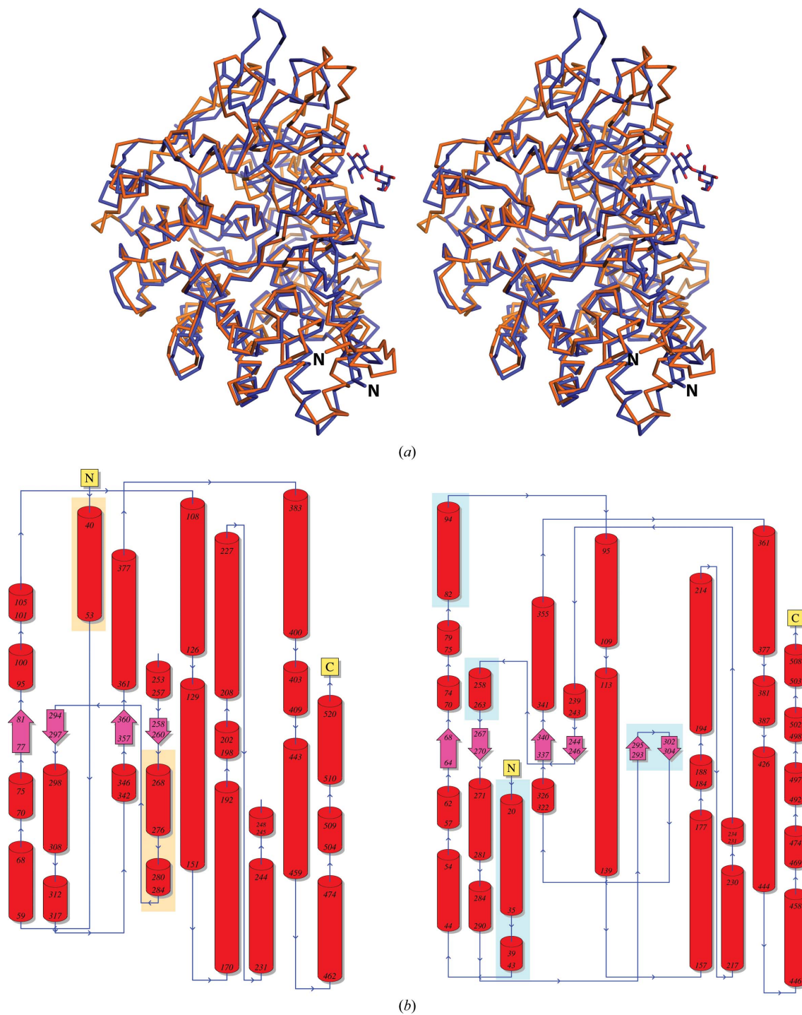
Figure 3 Structure comparison of BT_3984 and BT_1043. (a) Stereo ribbon diagram of BT_3984 (PDB code 3cgh; orange) and BT_1043 (PDB code 3ehn; blue). The N -acetylglucosamine sugar cocrystallized with BT_1043 is shown in ball-and-stick representation and the N -terminus of each protein is indicated. (b) Topology diagrams of BT_3984 (left) and BT_1043 (right). N -terminal and C -terminal regions and sequence limits for secondary-structure elements are indicated. Secondary-structure elements missing from either structure are indicated by orange- and blue-highlighted boxes for BT_3984 and BT_1043, respectively.
