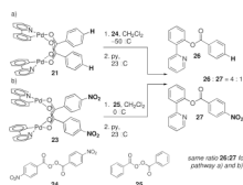
Scheme 3. Carboxylate scrambling on Pd(III) complexes is fast relative to C–O reductive elimination.
