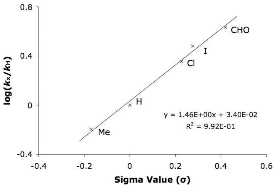
Figure 2. Hammett plot based on 7-benzo[ h ]quinoliny] substitution.
