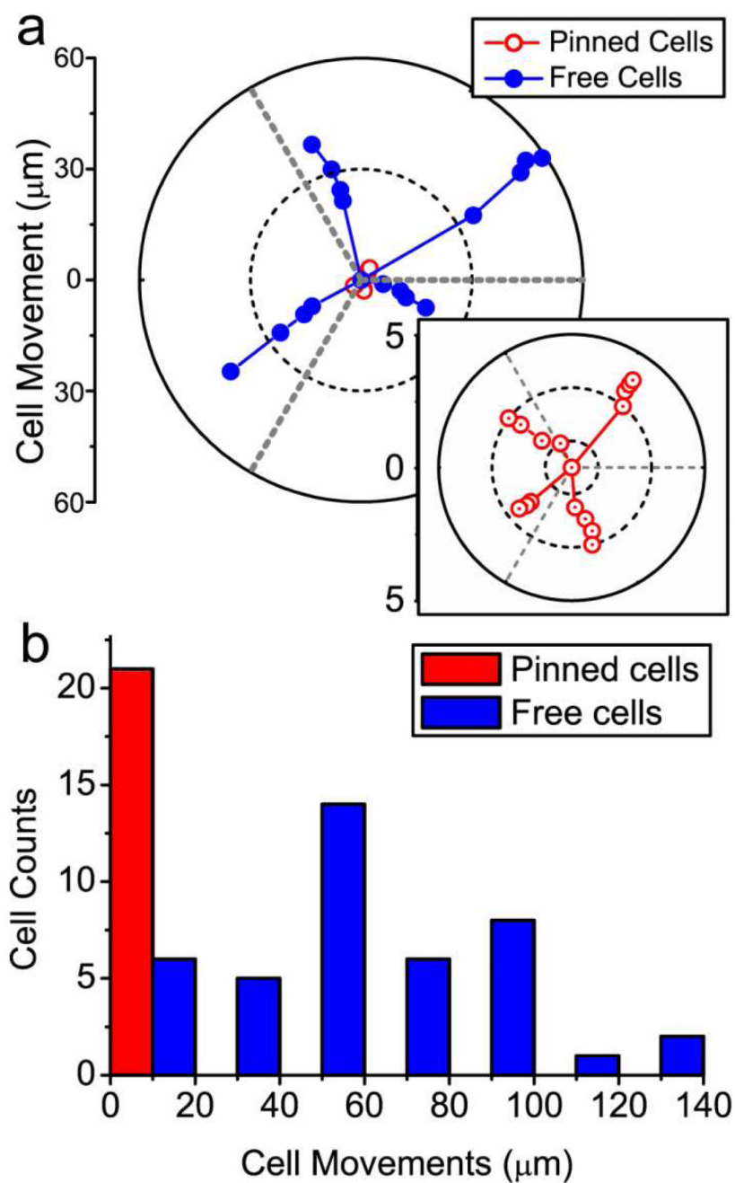
Figure 3. Statistics of cell migration over 5 days. (a) Typical movement traces of 4 nanopillar-pinned and 4 free-migrating neurons. Bottom right plot shows zoom-in of the nanopillar-pinned cell movements. While the free-migrating neurons explore \sim 60\mu\text{m} distances, the nanopillar-pinned cells move no more than 5\mu\text{m} . (b) Analysis of neuron movements over 42 free-moving and 21 nanopillar-pinned neurons show that nanopillars effectively stopped the migration of neurons.
