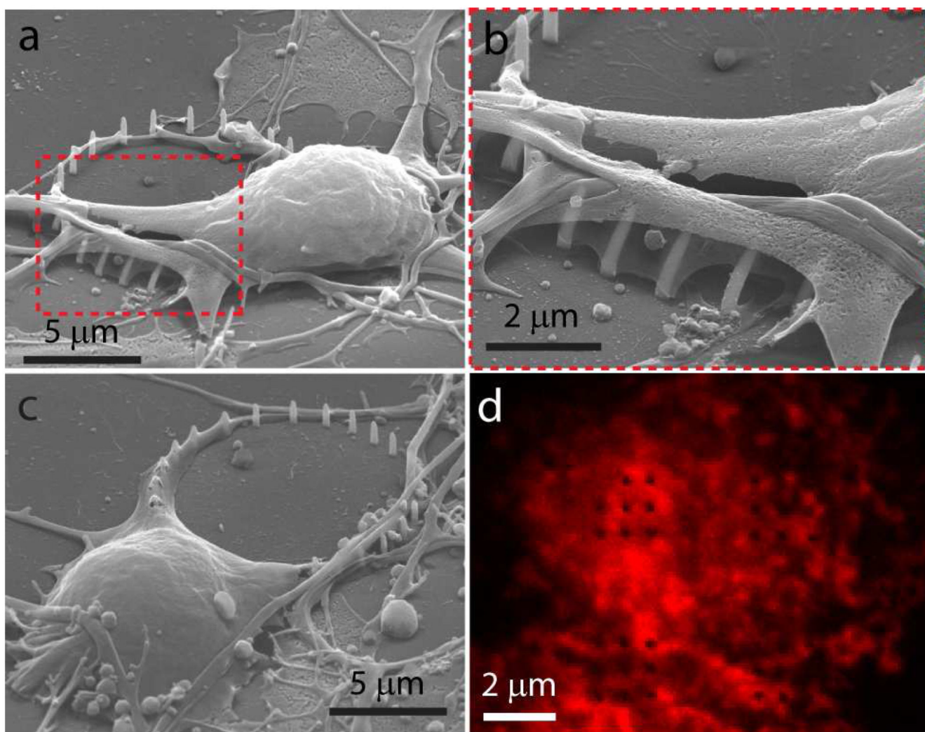
Figure 4. Examining the neuron-nanopillar interface by SEM and fluorescence microscopy. (a). An SEM image of a neuron growing atop a ring of nanopillars show close-contact between neurons and nanopillars. (b). Zoomed-in picture of (a) shows that cell membrane tightly wrapped around nanopillars. The interaction between the nanopillars and the neurons seem to exert forces on the nanopillars so as to bend some of them. (c). An SEM image of a neuron with one of its neurites preferentially growing along the ring-shaped nanopillar arrays. (d). Confocal microscope image of immunostained actin filaments shows that nanopillars (black dots) are imbedded in the cytoskeletal network.
