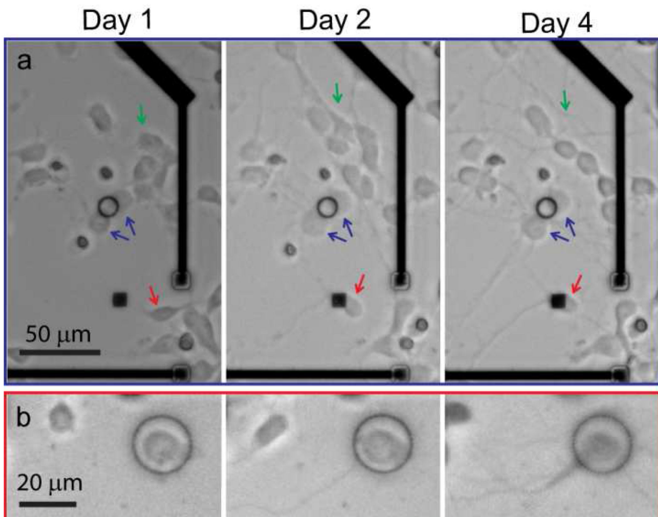
Figure 2. Migrations of cortical neurons are followed at 1 day, 2 days and 4 days after plating. Over this 4-day period, neurons that are in contact with nanopillar arrays display significantly reduced mobility compared with those that are not. On the other hand, all neurons show similar morphology, survival rate and neurite elongation rate. (a) Neurons that are not in contact with nanopillars (green arrows) are significantly more mobile over 4 days than those neurons in close contact with nanopillars (blue arrows). The red arrow points to a neuron that is very mobile in the first day on the flat surface before it comes into contact with a square nanopillar array and is arrested there. (b) A neuron initially plated inside a nanopillar ring is trapped inside.
