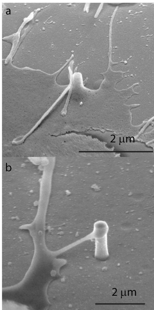
Figure 5. SEM of cells cultured on Si and SiO 2 nanopillar substrates. (a). An SEM image shows a SiO 2 pillar engulfed by the cell membrane. (b). An SEM image shows a protruding of a neuron reaching a Si nanopillar.
