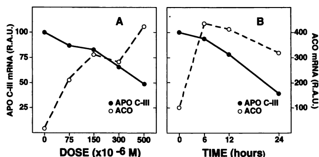
Figure 8. Dose- (A) and time- (B) dependent effects of fenofibrates on apo C-III and ACO mRNA levels in primary cultures of adult rat hepatocytes. Rat hepatocytes were isolated, treated either with the indicated doses for 24 h (A) or with 500 \mu M of fenofibrates for the indicated periods of time (B). Apo C-III and ACO mRNA levels were quantified as described in Methods.
