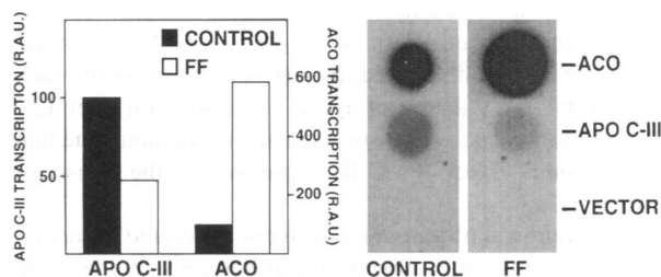
Figure 9. Fenofibrates regulate apo C-III and ACO gene expression at the transcriptional level. Nuclear run-on assays were performed on adult rat hepatocytes treated for 9 h with 500 \mu M of fenofibrates (FF) or vehicle (CONTROL) as described under Methods and analyzed by quantitative scanning densitometry.
