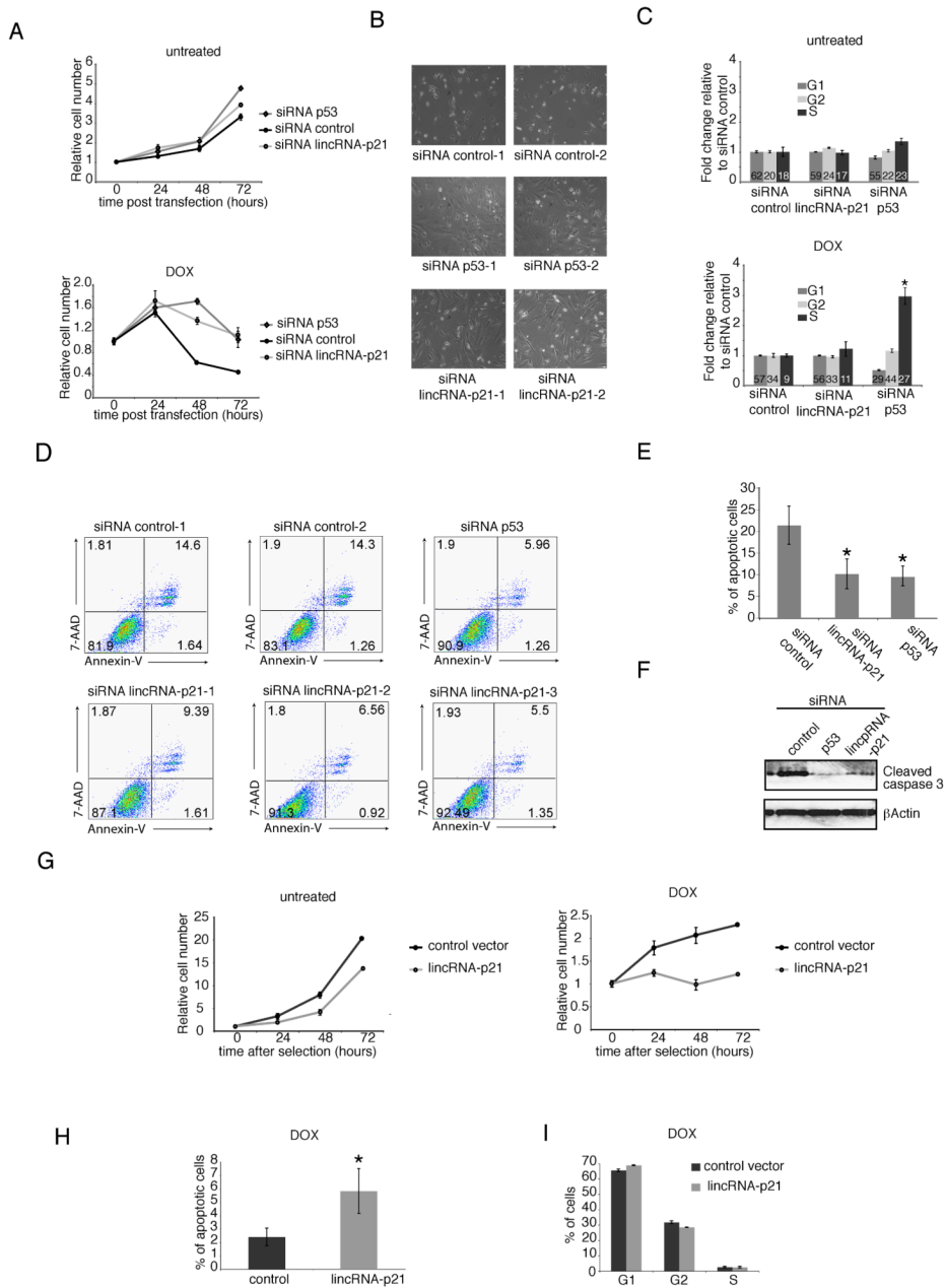
Fig 4. lincRNA-p21 is required for proper apoptotic induction
