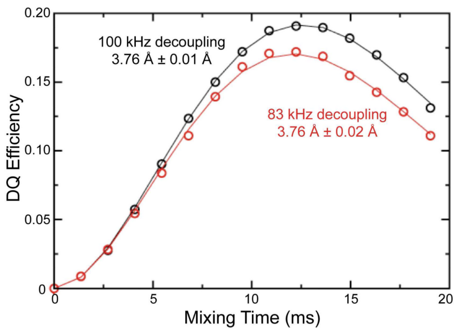
Figure 3. Double quantum buildup curves for 1,4- ^{13}\text{C} -succinate using 100 kHz (black circles) and 83 kHz (red circles) proton decoupling, and their corresponding best-fit simulations (black line and red line). The decrease in decoupling power results in a slight change in the best fit relaxation parameter, but the best fit distance parameter remains the same. These data and the data on the fibril samples were collected on a 360 MHz spectrometer using 4 mm rotors and \omega_r/2\pi = 5.882 kHz.
