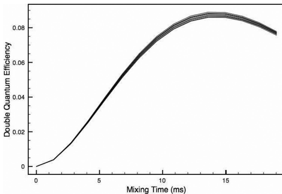
Figure 5. A set of 10 DQF-DRAWS simulations with random orientations of all four CSA tensors. The differences in these curves are smaller than the experimental errors so for simplicity we used the orientation of CSA tensors in which the most shielded axis of each tensor is parallel to the z-axis, while the spins lie in the x-y plane.
