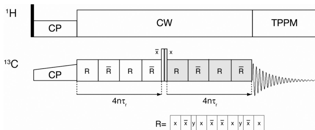
Figure 1. Pulse sequence for DQF-DRAWS experiment. Following cross-polarization, the DQF-DRAWS sequence (basic element R) is applied for a variable dipolar build up time for two conjugate periods. TPPM is used during acquisition, but CW decoupling is applied during the mixing sequence to avoid interference effects with TPPM. 74
