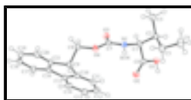
Fig. 1. A view of the molecular structure of (I), showing the atom labeling scheme. Displacement ellipsoids are drawn at the 50% probability level.
