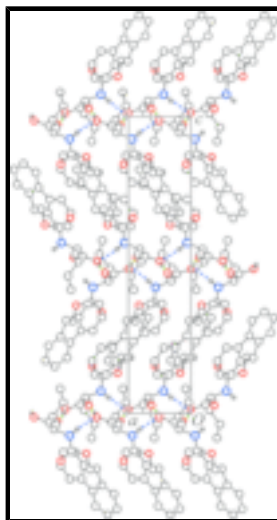
Fig. 2. A packing diagram of (I). The hydrogen atoms were omitted for clarity, except for those forming the hydrogen bonds. The hydrogen bonds are shown as blue and green broken lines for N—H...O and O—H...O bonds, respectively.
