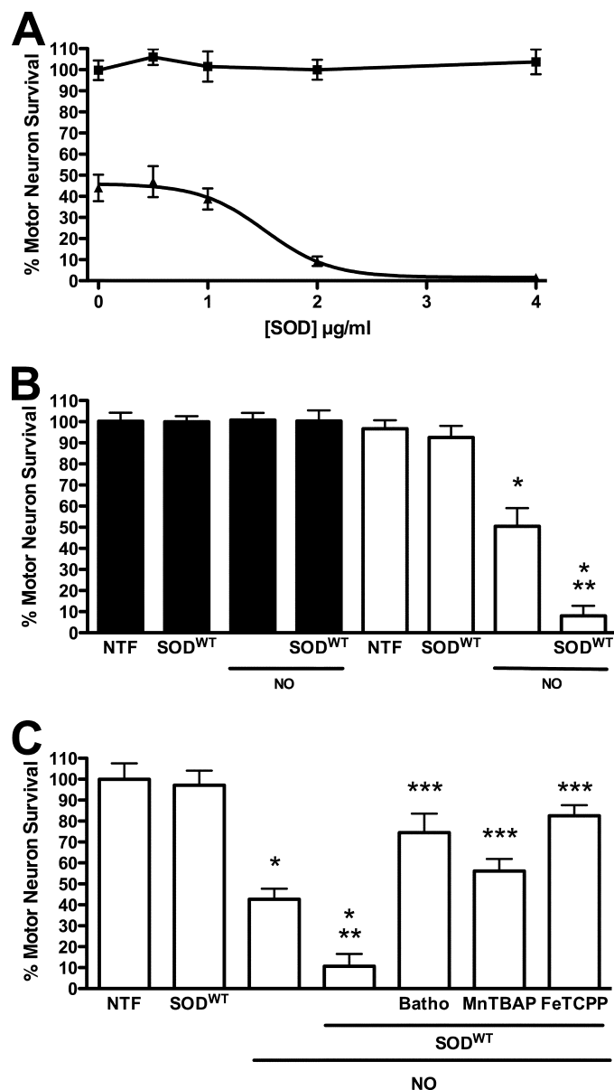
FIGURE 2. Cu,Zn-SOD WT enhances nitric oxide-induced SOD G93A motor neuron death. Motor neurons purified from transgenic rat for SOD G93A and nontransgenic littermates were plated in four-well plates and treated as indicated, and survival was determined 24 h later. A, motor neurons from transgenic rats for SOD G93A were incubated with growing concentrations of Cu,Zn-SOD WT alone (■) or in combination with DETANONOate (20 \mu M) (▲). The values representing the means \pm S.D. of at least three independent experiments performed in duplicate were fitted to a sigmoid curve with EC 50 = 1.5 \pm 0.15 \mu g (95% confidence interval (C.I.) 1.20 to 1.80) and R 2 = 0.934. B, motor neurons isolated from SOD G93A (open bars) and from nontransgenic littermates (filled bars) were incubated with 20 \mu M DETANONOate (NO), Cu,Zn-SOD WT (1 \mu g), or the combination of both treatments. The values are the means \pm S.D. of at least three independent experiments performed in quadruplicate. The values were analyzed by two-way ANOVA followed by Bonferroni's multiple comparison test. *, p < 0.01 versus transgenic NTF. **, p < 0.01 versus transgenic incubated with NO alone. C, motor neurons from transgenic rat were incubated with SOD WT released using Chariot, alone or in combination with 20 \mu M DETANONOate (NO). Cultures treated with SOD WT and DETANONOate were also incubated with the copper chelator bathocuproine (50 \mu M, Batho), and the superoxide and peroxynitrite scavengers MnTBAP (100 \mu M) and FeTCPP (10 \mu M). The values are the means \pm S.D. of three independent experiments performed in duplicate. The values were analyzed by ANOVA followed of Bonferroni's multiple comparison test. *, p < 0.05 versus NTF. **, p < 0.05 versus NO alone. ***, p < 0.05 versus NO plus SOD.
