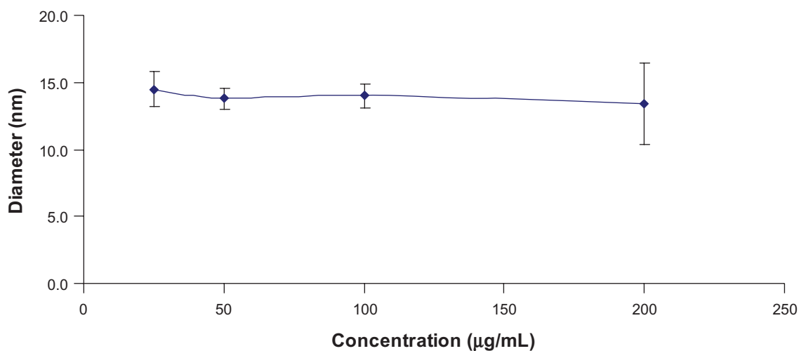
Figure 3 Critical micellar concentration of PGG-PTX nanoconjugate. The DLS could not detect the particle size of PGG-PTX solution below 25 µg/mL. The critical micellar concentration was assumed to be about 25 µg/mL in saline at 25°C. The results are expressed as means ± SD (n = 3). Abbreviation: DLS, dynamic light scattering.
