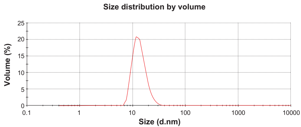
Figure S6 PGG-PTX (2,000 \mu\text{g/mL} ) in saline. Diameter = 13.7 nm; PDI = 0.404.
