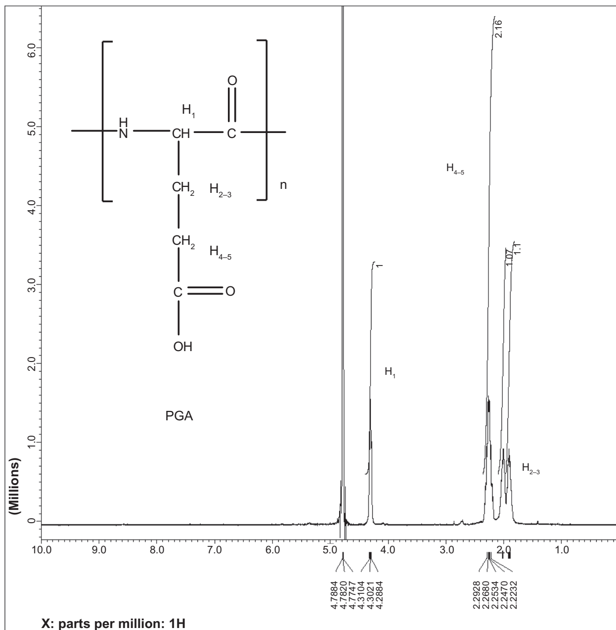
Figure S1 1 H-NMR spectra of PGA-PGG, and PGG-PTX.
