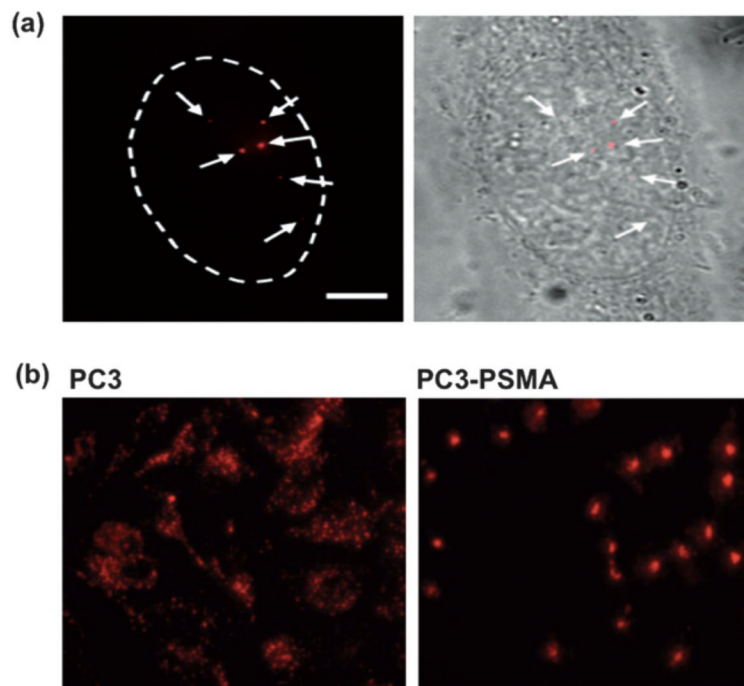
Fig. 3. Cellular delivery of QDs. (a) Monodispersed QDs can be delivered by microinjection. The single nature of QDs can be validated by the blinking phenomenon. 67 The ability to deliver controlled amounts of QDs with spatial and temporal precision is particularly useful for single-molecule studies. (b) The labeling pattern of QDs is phenotype-dependent. Unlabeled QDs are found aggregated throughout the cytoplasm in the PC3 cells, as previously observed along the endosomal pathway. Strikingly, a single clump of QDs is localized around the perinuclear region of PC3-PSMA cells. 69 As a result, cancer phenotypes can easily be identified by the contrasting labeling pattern of QDs. Figures reprinted with permission from the American Chemistry Society and Wiley-VCH Verlag GmbH & Co.
