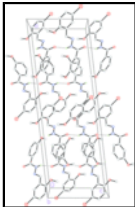
Fig. 2. The packing diagram of (I), viewed along the b axis. Hydrogen bonds are shown as dashed lines.
