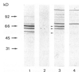
Figure 2. Western blots on the membrane proteins of E. coli expressing the human β 1 -adrenergic receptor. (Lane 1) Proteins revealed with affinity-purified rabbit anti-β 1 -peptide antibodies (15). (Lane 2) Affinity-purified rabbit anti-β 1 -peptide antibodies preincubated with the peptide before incubation with the blotted proteins. (Lane 3) Proteins revealed
