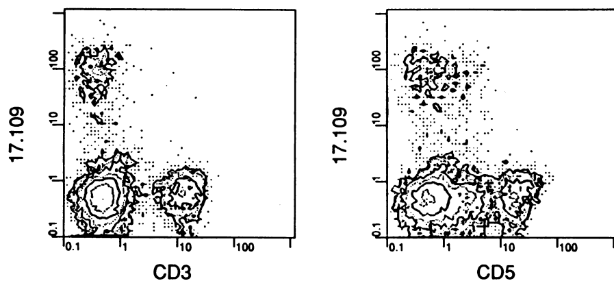
Figure 2. FACSscan immunofluorescence analyses of tonsillar lymphocytes labeled with PE-conjugated 17.109 and fluorescein-conjugated anti-CD3 ( left ) or fluorescein-conjugated anti-CD5 ( right ). Numbers correspond to the relative red ( ordinate ) or green ( abscissa ) fluorescence intensity of the cells when excited at 488 nm.
