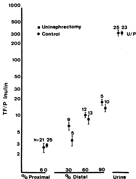
FIGURE 2 Summary of tubular fluid-to-plasma inulin concentration ratios (TF/P) as a function of tubular length in control and uninephrectomized rats. The mean \pm standard error are represented. n, number of observations. The control and experimental values were not significantly different.
