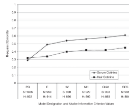
Figure 1. Predictive ability of increasingly complex models of determinants of serum cotinine and hair cotinine. R^2 values were estimated from ordinary least squares linear regression using data from the 12-month visit of the Cincinnati Asthma Prevention Study (2000–2003). Akaike Information Criterion values for models predicting serum cotinine (S) and hair cotinine (H) were estimated from linear mixed models using all available study data. Models included variables that met inclusion criteria as listed in Table 3, from the following additional groups: PQ, parent questionnaire, E, environmental measures, HV, housing and ventilation characteristics, NH, non-home places, Child, child characteristics, SES, family social class characteristics.
