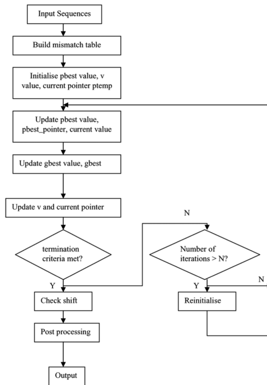
Figure 2. Overview of PSO-motif algorithm
