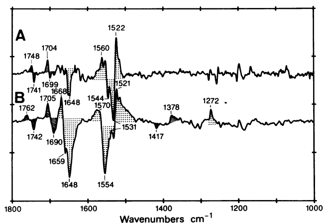
FIG. 3. A, Subtraction of the BR – L difference spectra of the wild type and the mutant; B, corresponding subtraction of the BR – M difference spectra. For details see text.
