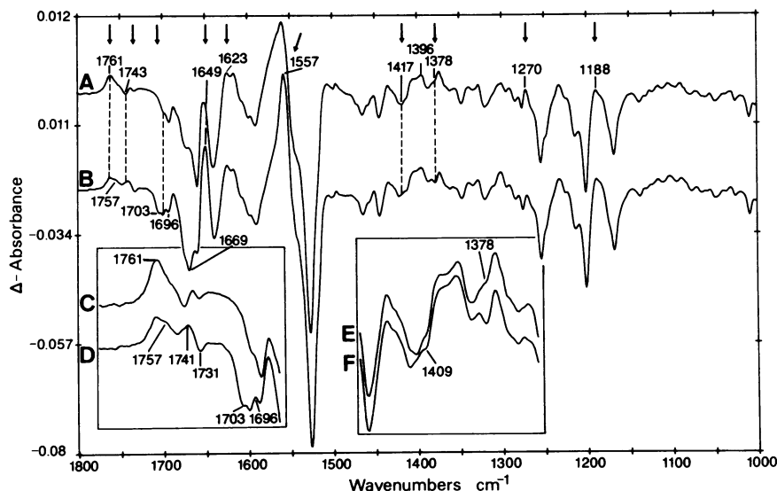
FIG. 2. BR - M difference spectra of bacteriorhodopsin taken at 272 K in \text{H}_2\text{O} with 2 \text{cm}^{-1} spectral resolution. The M intermediate is stabilized under photostationary conditions. Thereby small contributions of the N intermediate are present, but in the same ratio in both samples, as indicated in the fingerprint region. A, wild type; B, mutant; C, expansion of A from 1800 to 1680 \text{cm}^{-1} ; D, expansion of B from 1800 to 1680 \text{cm}^{-1} ; E, expansion of A from 1450 to 1350 \text{cm}^{-1} ; F, expansion of B from 1450 to 1350 \text{cm}^{-1} .
