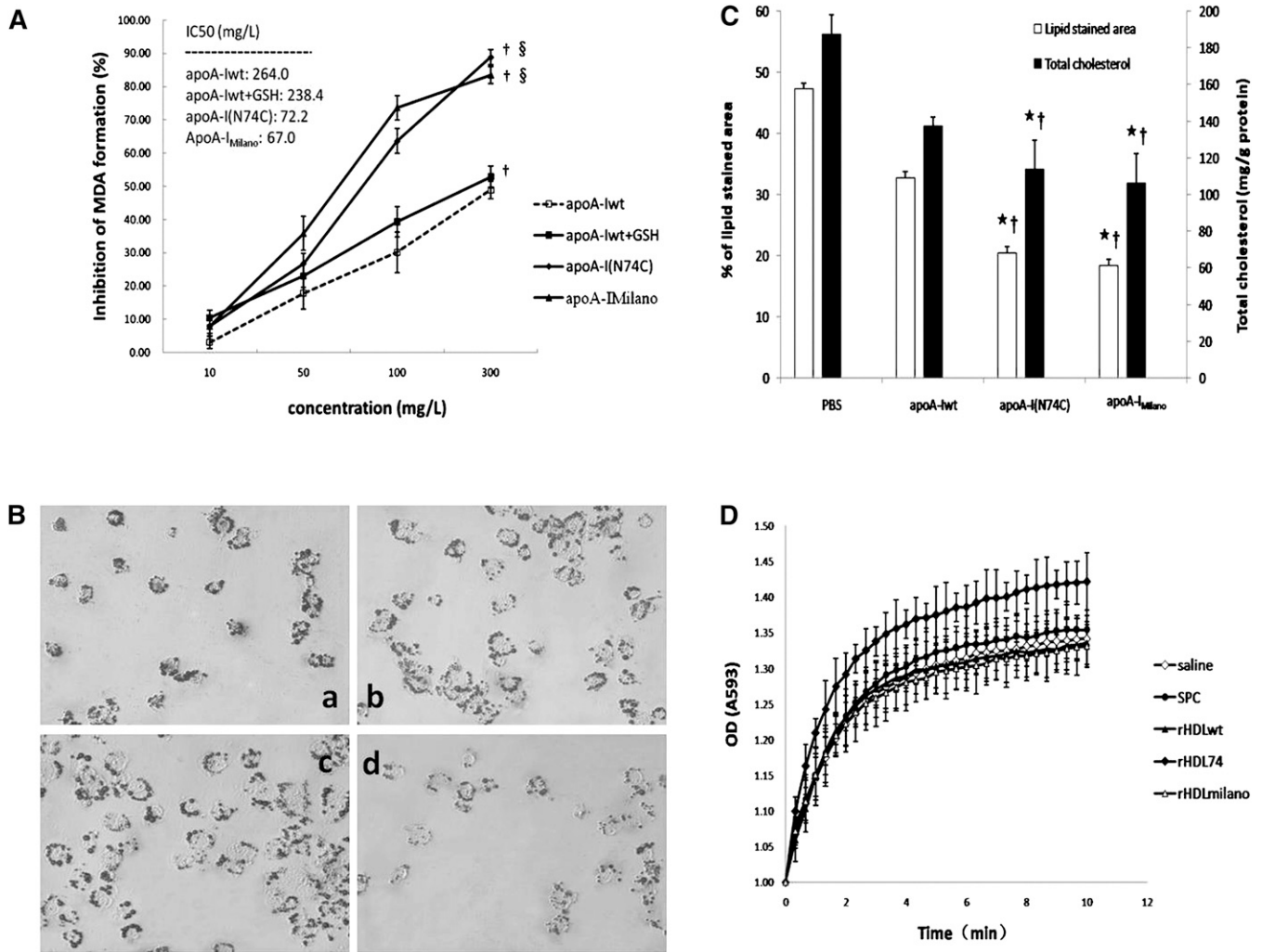
Fig. 1. Antioxidant activity of apoA-I(N74C) in lipid-free state in vitro and in lipid-bound state in vivo. A: Potent inhibitory effect of recombinant apolipoproteins against LDL oxidation in the presence of 5 \mu M CuSO 4 in vitro. Freshly prepared LDL (100 mg/l) was incubated with each apolipoprotein (10–300 mg/l) for 4 h at 37°C. After incubation, samples were assayed for MDA formation and expressed as percentage of inhibition relative to the Cu 2+ -only controls. The IC 50 values were calculated from the linear slopes of the graphs. To preclude the effects of thiols induced by cysteine mutation, the same molar concentrations of GSH as the apolipoproteins tested were added to apoA-Iwt reaction system and analyzed the antioxidant effects. B: The Oil Red O staining in THP-1-derived macrophages treated with PBS at 40 \times magnification: (a) apoA-Iwt (control); (b) apoA-Iwt + GSH; (c) apoA-I(N74C); and (d) apoA-I Milano . C: Quantitative analysis of the intracellular lipid accumulation in THP-1-derived macrophages. The areas of Oil Red O staining were calculated using the Image-Pro Plus software. To verify the data of lipid staining area, the intracellular total cholesterol level expressed as the ratio between total cholesterol and total protein was analyzed. D: Antioxidant ability of mice serum measured by FRAS. Absorption of rHDL74-injected serum at 593 nm for up to 10 min exhibited of up to 42% more than the initial values. Data are expressed as mean \pm SD. * P < 0.05 versus PBS; † P < 0.05 versus apoA-Iwt; § P < 0.01 versus apoA-Iwt + GSH. Apo, apolipoprotein; apoA-I(N74C), apolipoprotein A-I(N74C); apoA-Iwt, wild-type apoA-I; FRAS, ferric reducing ability of serum; GSH, L-glutathione; rHDL, recombinant HDL; IC 50 , half-maximal inhibitory concentration; MDA, malondialdehyde.
