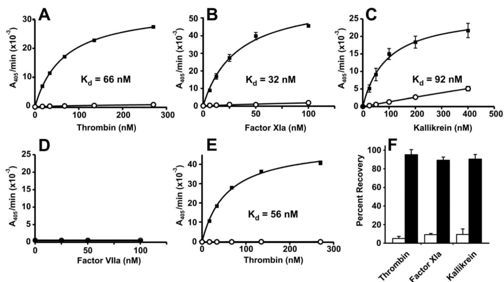
Figure 3. Binding of clotting proteases to immobilized polyP. (A-C) PolyP HMW was coupled via EDAC to Amine Surface microplate wells, which were then used to quantify the binding of (A) thrombin, (B) factor XIa, (C) kallikrein, or (D) factor VIIa. (E) Biotinylated polyP HMW was immobilized on streptavidin-coated microplate wells, which were then used to quantify thrombin binding. For panels A-E, solid squares are binding data after background subtraction, while open circles are background binding (from wells without polyP); lines represent the single-site ligand binding equation fitted to the binding data, yielding the indicated K_d values. (F) PolyP HMW was coupled via EDAC to primary amine-containing Sepabeads. Thrombin (27 pmol), factor XIa (10 pmol), or kallikrein (10 pmol) were incubated with polyP-Sepabeads, after which the beads were collected and washed by centrifugation. Enzyme recovery was quantified in the flow-through (open bars) and high-salt eluates (closed bars), with recoveries calculated as percent of the starting material. Data are mean \pm S.E.M. ( n=3 ).
