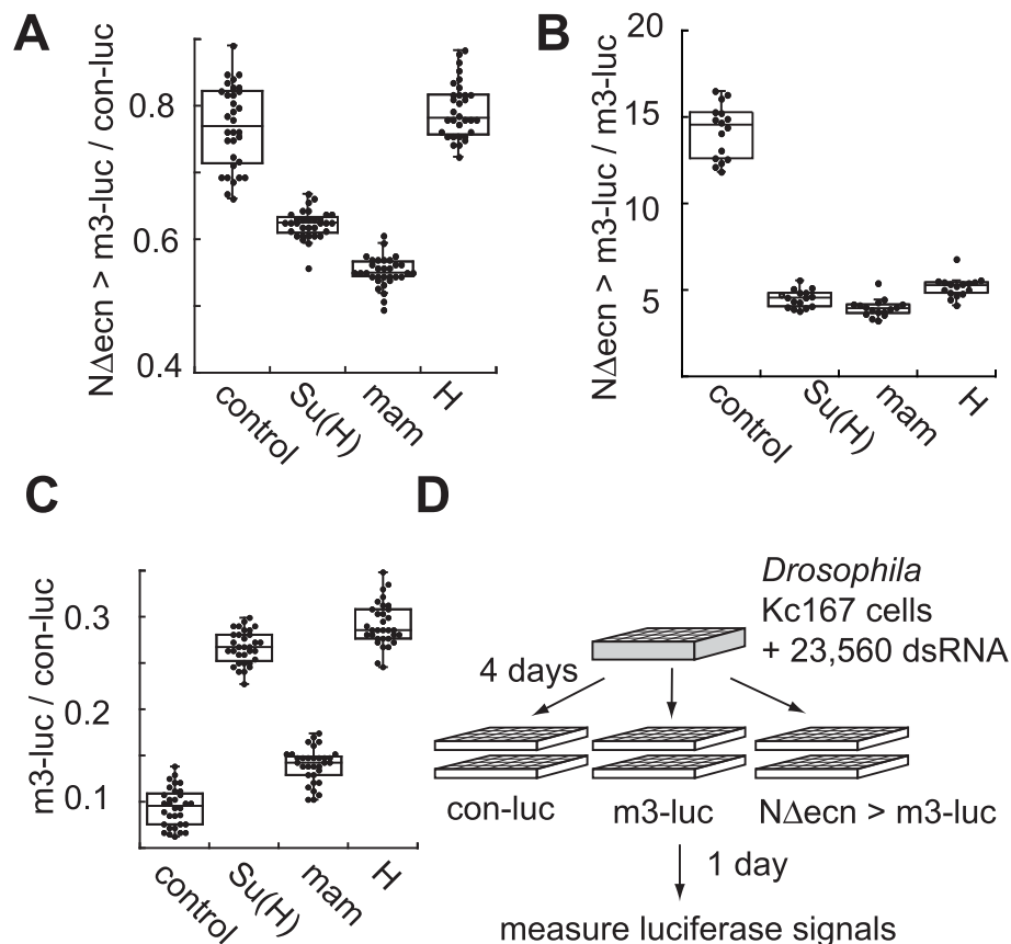
Figure 1 Validation of the Notch activity reporter and application for high throughput RNAi. Validation of the m3-luc reporter by RNAi targeting of known Notch pathway components. Notch induced E(spl)m3 signal normalized against A . the control viral promoter or B . uninduced E(spl)m3 promoter transcription. C . Uninduced E(spl)m3 promoter expression normalized by control promoter. For each dsRNA, 32 independent wells were measured in a 384-well plate format. Each box encloses 50% of the data with the median value displayed. The error bars mark the full range excluding the shown outliers. D . Schematic of the automated high throughput screen in 384-well plates. Drosophila Kc167 cells were incubated with a unique dsRNA per well. After a four day incubation, the cells were split into three different transfection mixes in duplicate. Firefly luciferase signals were read 24 h after transfection.
