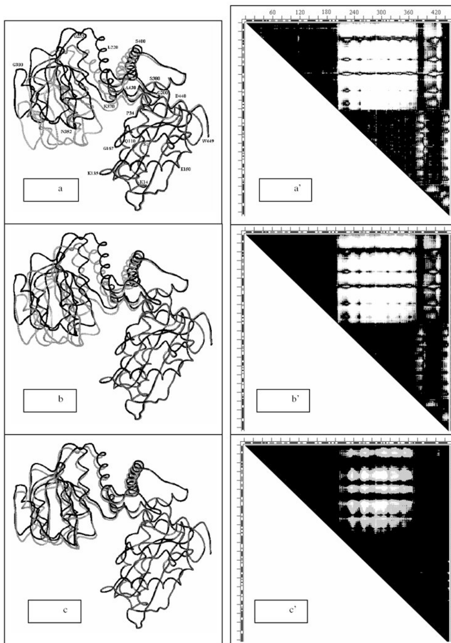
Fig. 12. a-c. Three snapshots (#1, #40 and #80 out of 100 total) from elastic coarse grained dynamics movie of the motion pathway of Glu dehydrogenase for each of conformation 1bgv (gray) changing into 1hrd (black) which is completed in snapshot #100). In all snapshots rigid fragments 1-204 are superimposed. Residue numbers (on 'a' only) directly refer to the black wire (1hrd) and only approximately to the nearby gray wire (1bgv). a'-c'. Three DDM-s 1hrd1bgv where conformation of 1bgv is taken to correspond to the three snapshots (#1, #40 and #80) from Fig.14a-c. DDM for snapshot #100 would be completely black because 1aam would completely change its conformation to 1hrd.
