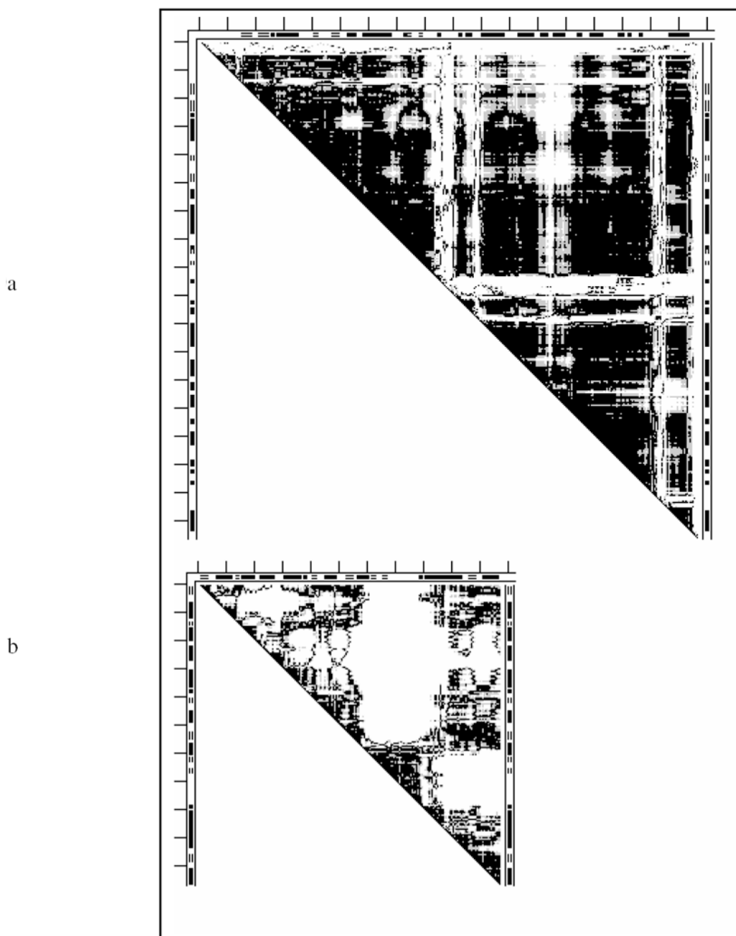
Fig. 9. DDMs for two kinases: a) 1erk2erk (signal regulated kinase); b) 4ake1ank (adenylate kinase) For notations see legend to Fig. 1.
