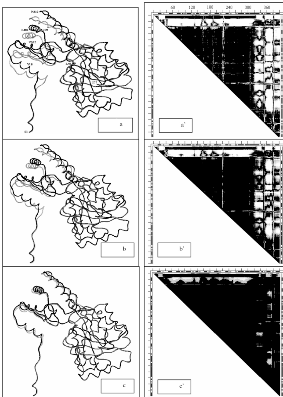
Fig. 11. a-c. Three snapshots (#1, #40 and #80 out of 100 total) from elastic coarse grained dynamics movie of the motion pathway of Asp aminotransferase for each of conformations of 1ama (gray) changing into 9aat (black), which is completed in snapshot #100. In all snapshots rigid fragments 228-305 are superimposed. Wire rendering is done with MOLE (G.P. Privalov, gpriv@axonx.com); Residue numbers (on 'a' only) directly refer to the black wire (9aat) and only approximately to the nearby gray wire (1ama). a'-c'. Three DDM-s 9aat1ama where the conformation of 1ama is taken to correspond to the three snapshots (#1, #40 and #80) from panels a-c. DDM for snapshot #100 would be completely black because 1aam would completely change its conformation to 9aat.
