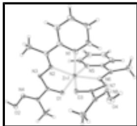
Fig. 1. 1 A view of compound 1 , with displacement ellipsoids shown at the 40% probability level.
