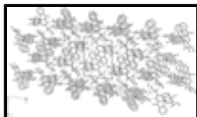
Fig. 2. A packing diagram for 1 viewed in projection down the a axis. Hydrogen bonds are indicated by dashed lines; H atoms are omitted for clarity.
