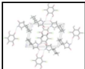
Fig. 2. Packing diagram of the title compound, (I), viewed down the a axis. Dashed lines indicate strong N—H···O and O—H···O intermolecular hydrogen bonds linking the C_9H_{15}NO and C_6H_2Cl_2O_4 molecules into an infinite O—H···O—H···O—H chain network along the b axis in (011).
