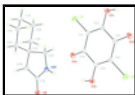
Fig. 1. Molecular structure of C_9H_{15}NO.C_6H_2Cl_2O_4 showing the atom labeling scheme and 50% probability displacement ellipsoids. H atoms are presented as small circles of arbitrary radius.
