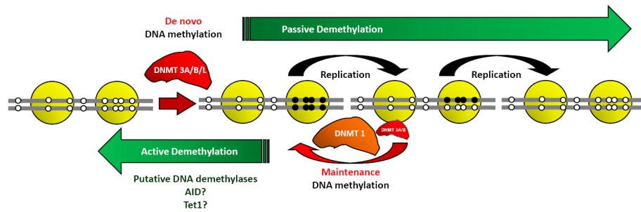
Figure 2. DNA methylation and demethylation
