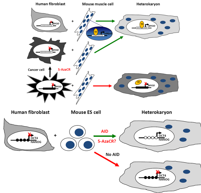
Figure 1. Cell fusion experiments showing the importance of DNA methylation as an epigenetic barrier for reprogramming
