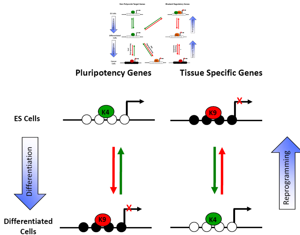
Figure 3. Epigenome landscaping during differentiation and carcinogenesis
