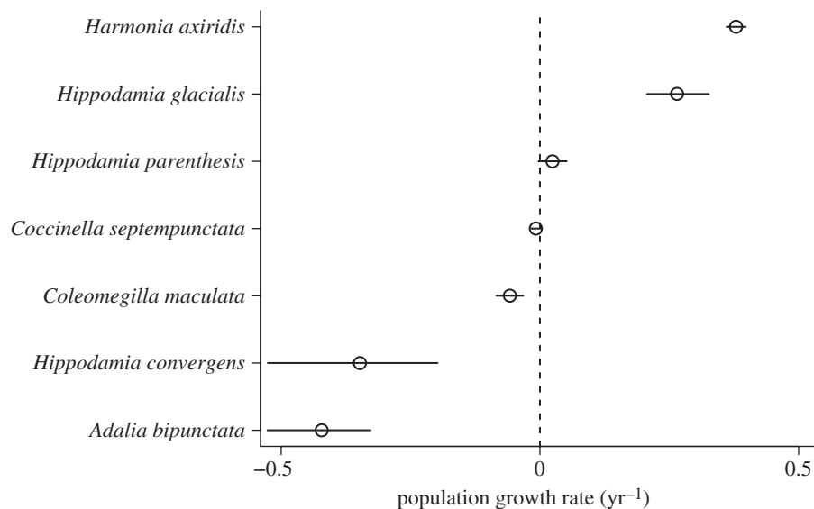
Figure 7. Hierarchical model estimates of r_b , the intrinsic rate of increase ( = \ln(\lambda) ) for seven species of grassland insects. Details as in figure 5.
