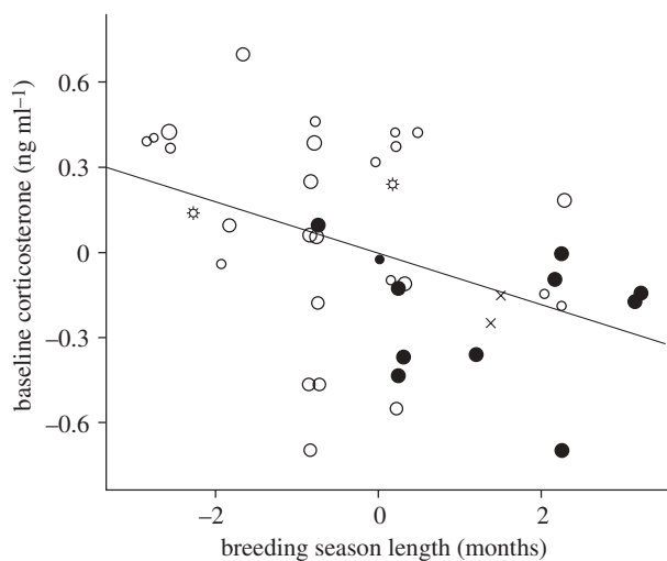
Figure 1. Partial regression plot showing inverse relationship between baseline corticosterone concentrations (Cort0; \text{ng ml}^{-1} ) and breeding season length (months). Data are displayed as unstandardized residuals after controlling for body mass in a linear regression model. The figure shows the largest dataset used in this study. Larger symbols denote own original dataset, smaller symbols refer to published data. Environments are coded as: open circles, mesic; filled circles, tropical; crosses, arid; stars, cold (arctic or alpine).
