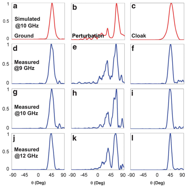
Figure 6 | The simulated and measured electric fields in the far region.
