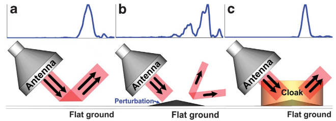
Figure 5 | Three situations for measurements and simulations and the predicted far-field patterns. (a) The flat ground plane, with a single-peak reflection at the mirror-reflecting direction of the incident wave. (b) The ground plane with a cone-shaped metallic perturbation, with multi-peak reflections. (c) The ground plane with both perturbation and 3D cloak, with a single-peak reflection at the mirror-reflecting direction of the incident wave. The electric field amplitude in the top half of the panels is normalized to unity.
