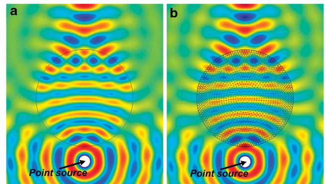
Figure 3 | Full-wave simulation results of electric fields inside and outside the metamaterials. The calculations are performed for the circular continuous-material and drilled-hole metamaterial plates under the excitation of a 2D point source at 10 GHz. Both plates have a radius of 62.5 mm and a thickness of 3 mm, and are placed in a planar waveguide. Hence, the simulations can be performed using 2D models (TE polarization). (a) Continuous-material plate. (b) Drilled-hole metamaterial plate.
