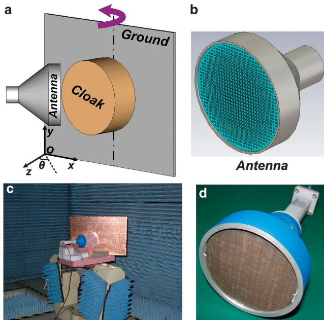
Figure 4 | Measurement system of the 3D ground-plane cloak. A metamaterial lens antenna is used to transmit a narrow-beam plane wave in the near-field region, and a normal X-band rectangular horn antenna is used to receive the far-field scattered electric fields. (a) The demonstration of measurement. (b) The sketch of the metamaterial gradient index lens antenna. The green surface is made of metamaterials. (c) The actual measurement system in a fully anechoic chamber. (d) The photograph of the metamaterial antenna.
