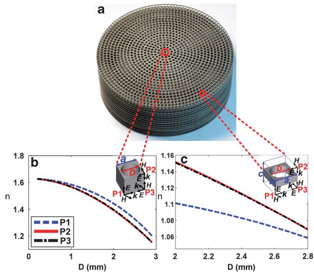
Figure 2 | Unit cells used in the design of the cloak and the relation of geometry to electric field polarization. (a) The designed ground-plane cloak. (b) The 3 \times 3 \times 3 mm 3 drilled-hole unit cell, in which a = 3 mm, and the relations between effective index of refraction and unit-cell geometry for different polarized incident electric fields at 10 GHz. P1, P2 and P3 are three orthogonal polarizations, E and H are the electric and magnetic field and k is the wave vector of the incident radiation. (c) The 3 \times 3 \times 1 mm 3 drilled-hole unit cell, in which a = 3 mm, b = 3 mm and c = 1 mm, and the relations between effective index of refraction and unit-cell geometry for different polarized incident electric fields at 10 GHz.
