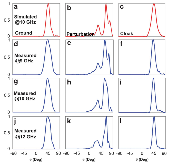
Figure 7 | The simulated and measured electric fields in the far region.
