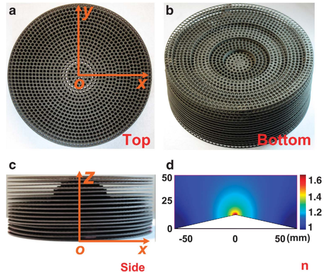
Figure 1 | Three-dimensional microwave ground-plane cloak and its refractive index distribution. (a) Top view of the cloak. (b) Bottom view of the cloak. (c) Side view of the cloak. (d) The distribution of refractive index in the x - z plane. The material parameters of the whole cloak are obtained by rotating the x -to- z -plane pattern around the z axis.
